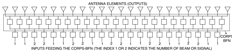
Figure 5. System of 24 radiators and 22 input ports with 12 complex inputs to control 24 antennas (beam # 1) and 10 complex inputs to control 20 antennas (beam # 2). Reproduced courtesy of the Electromagnetics Academy.
