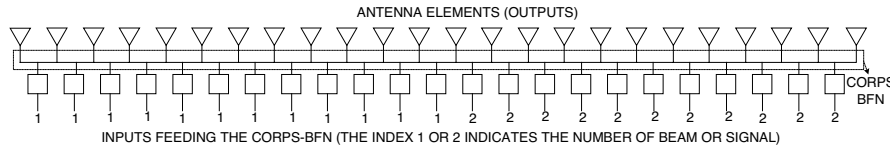
Figure 3. System of 24 radiators and 23 input ports with 12 complex inputs to control 13 radiators (beam # 1) and 11 complex inputs to control 12 antennas (beam # 2). Reproduced courtesy of the Electromagnetics Academy.
