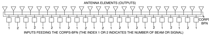
Figure 4. System of 24 radiators and 23 input ports with 12 complex inputs to control 24 antennas (beam # 1) and 11 complex inputs to control 22 antennas (beam # 2). Reproduced courtesy of the Electromagnetics Academy.
