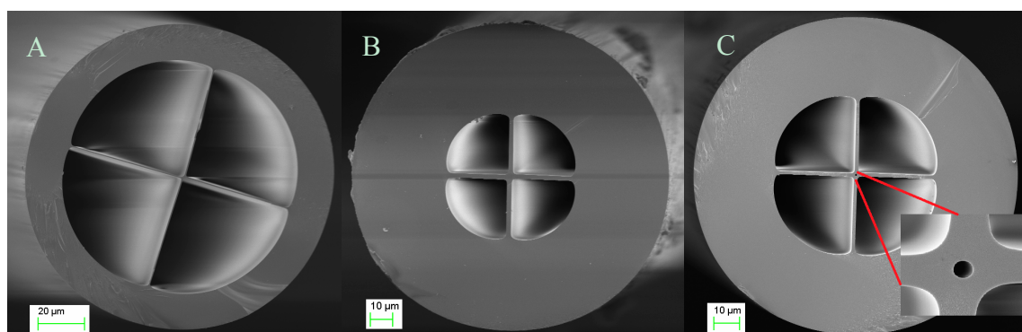
Figure 1. MOF-1 (A), MOF-2 (B) and MOF-3 (C) cross section. In the Figure (C), it can be appreciated a detail of the hole located in the center of the optical fiber.
