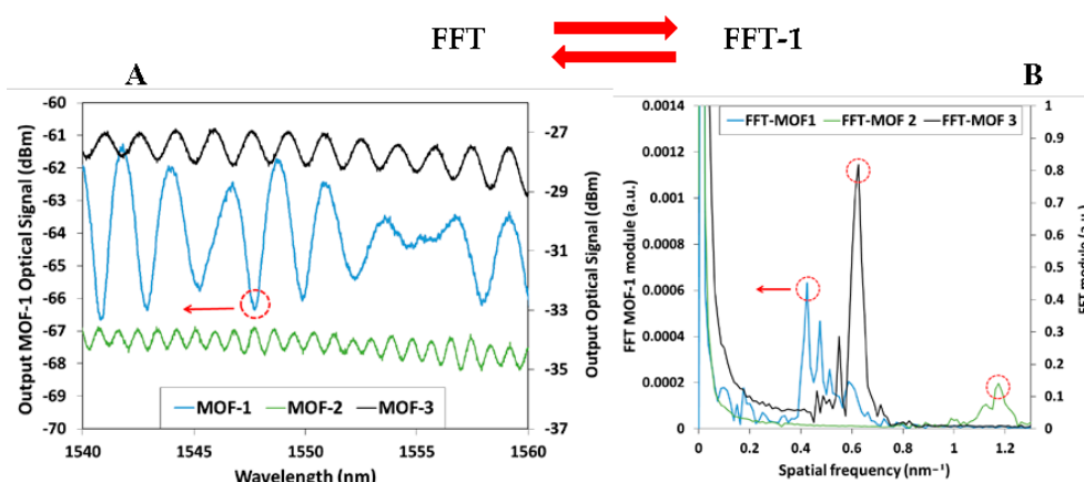
Figure 3. (A) Optical spectrum of MOFs and their FFTs (B); in both figures, the vertical left axel is applied for MOF-1 and the right axel for MOF-2 and MOF-3.
