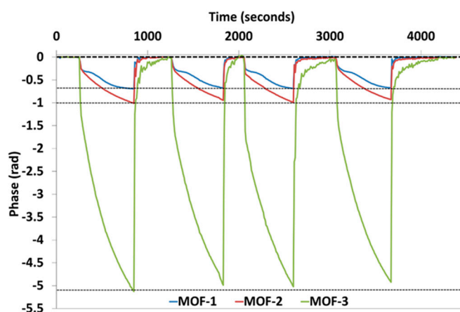
Figure 4. Phase responses of the three sensors for saturated atmospheres of ethanol.
