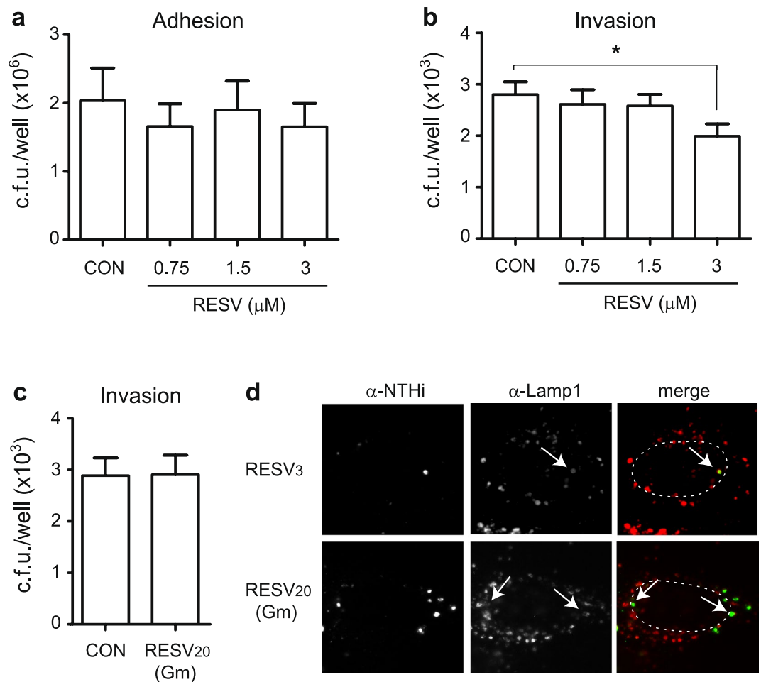
Figure 2. A resveratrol sub-inhibitory concentration lowers NTHi375 invasion of A549 human respiratory epithelial cells. Controls (CON): in adhesion and invasion assays (a and b, respectively), cells did not receive resveratrol (RESV), but did receive vehicle solution (DMSO) prior and during bacterial contact; in invasion assay (c), cells received vehicle solution during gentamicin treatment. Effect of resveratrol sub-inhibitory concentrations on NTHi375 adhesion to- (a) and invasion of (b) A549 cells. Cells were pre-treated with resveratrol 0.75, 1.5, or 3 \mu\text{M} for 4 h, and the polyphenol was maintained during infection. Bacterial adhesion was comparable for resveratrol-treated and control (CON) cells. Mean numbers of NTHi375 entry into cells treated with resveratrol 3 \mu\text{M} were significantly lower than those obtained for control (CON) cells ( p < 0.05 ). (c) Resveratrol effect on intracellular NTHi375. A549 cells were infected and resveratrol 20 \mu\text{M} was added during cell incubation with gentamicin (Gm). Resveratrol did not reduce the number of intracellular bacteria. (d) Subcellular location of NTHi375 inside A549 cells shows co-localization with Lamp-1 endosomal marker. NTHi was stained with rabbit \alpha\text{-NTHi} and Alexa 488-conjugated donkey \alpha\text{-rabbit} (green) antibodies. Lamp-1 was stained with mouse \alpha\text{-Lamp-1} and donkey \alpha\text{-mouse} conjugated to RRX (red) antibodies. A549 cells were pre-treated with resveratrol 3 \mu\text{M} for 4 h, which was maintained during infection (upper panels); alternatively, A549 cells were infected for 2 h and resveratrol 20 \mu\text{M} was added during cell incubation with Gm (lower panels). Representative images are shown, taken at 1 h post-Gm. Host cell nuclei location is indicated with dashed lines. Bacteria:Lamp-1 co-localization is indicated with arrows.
