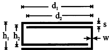
FIG. 2. SSRR drawn to scale d_2 = d_1 - s - w is the overlapped length between the long arms. h_2 = h_1 - s - 2w is the mean distance between long strips. Dimensions of the real SSRR in the experiment: d_1 = 5 mm, h_1 = 1.47 mm, s = 0.127 mm, w = 0.076 mm. The periodicity of the array is a = 1.99 mm.
