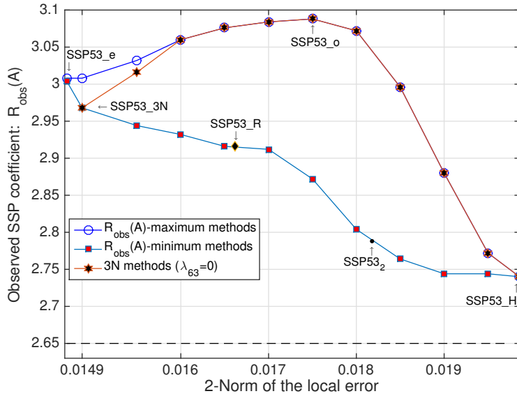
Figure 2: Observed SSP coefficient R_{obs}(\mathbb{A}) vs. 2-norm for the local error for optimal SSP(5,3) methods (17-18).
