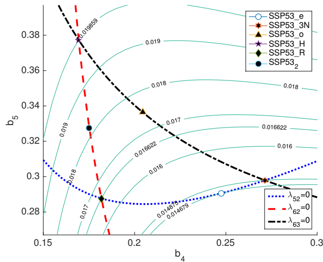
Figure 1: (b_4, b_5) -region for optimal SSP(5,3) methods (17-18) and level sets of the local error norm \|C_{err}\|_2 . The six optimal SSP(5,3) methods considered in this paper are shown with different symbols.
