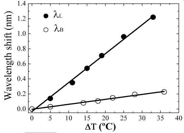
Figure 4. Wavelength shift as a function of temperature change for the wavelengths \lambda_L and \lambda_B (first structure).
