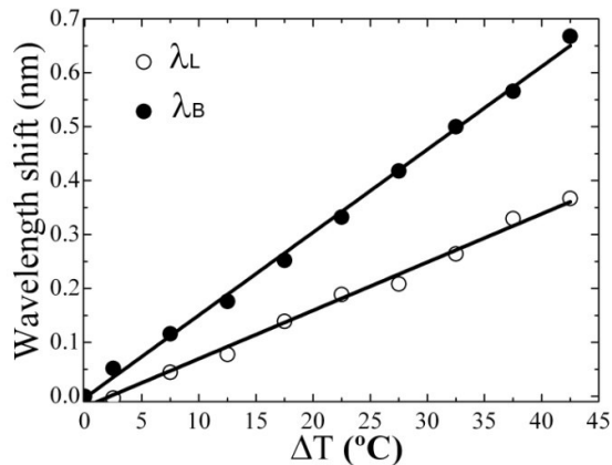
Figure 6. Wavelength shift as a function of temperature change for the wavelengths \lambda_L and \lambda_B (second structure).
