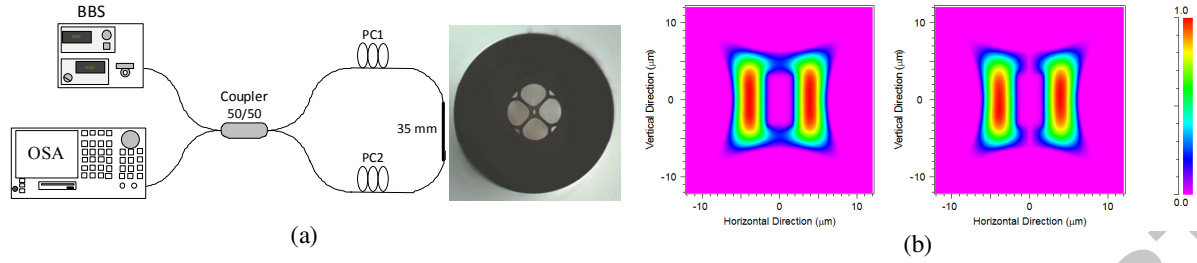
Figure 1. (a) Schematic diagram of the sensing system (a photograph of the clover microstructured fiber is also shown). (b) modeling of the light propagation in the microstructured fiber for two orthogonal polarizations.
