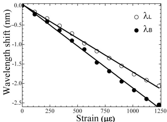
Figure 5. Wavelength shift as a function of strain change for the wavelengths \lambda_L and \lambda_B (second structure).
