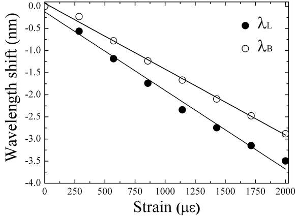
Figure 3. Wavelength shift as a function of strain change for the wavelengths \lambda_L and \lambda_B (first structure).
