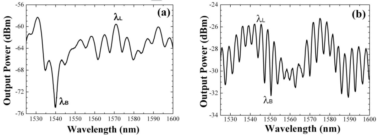
Figure 2. Output spectrum response of the fiber loop sensing structure using a clover microstructured fiber section with (a) 35 mm or (b) 89 mm length.
