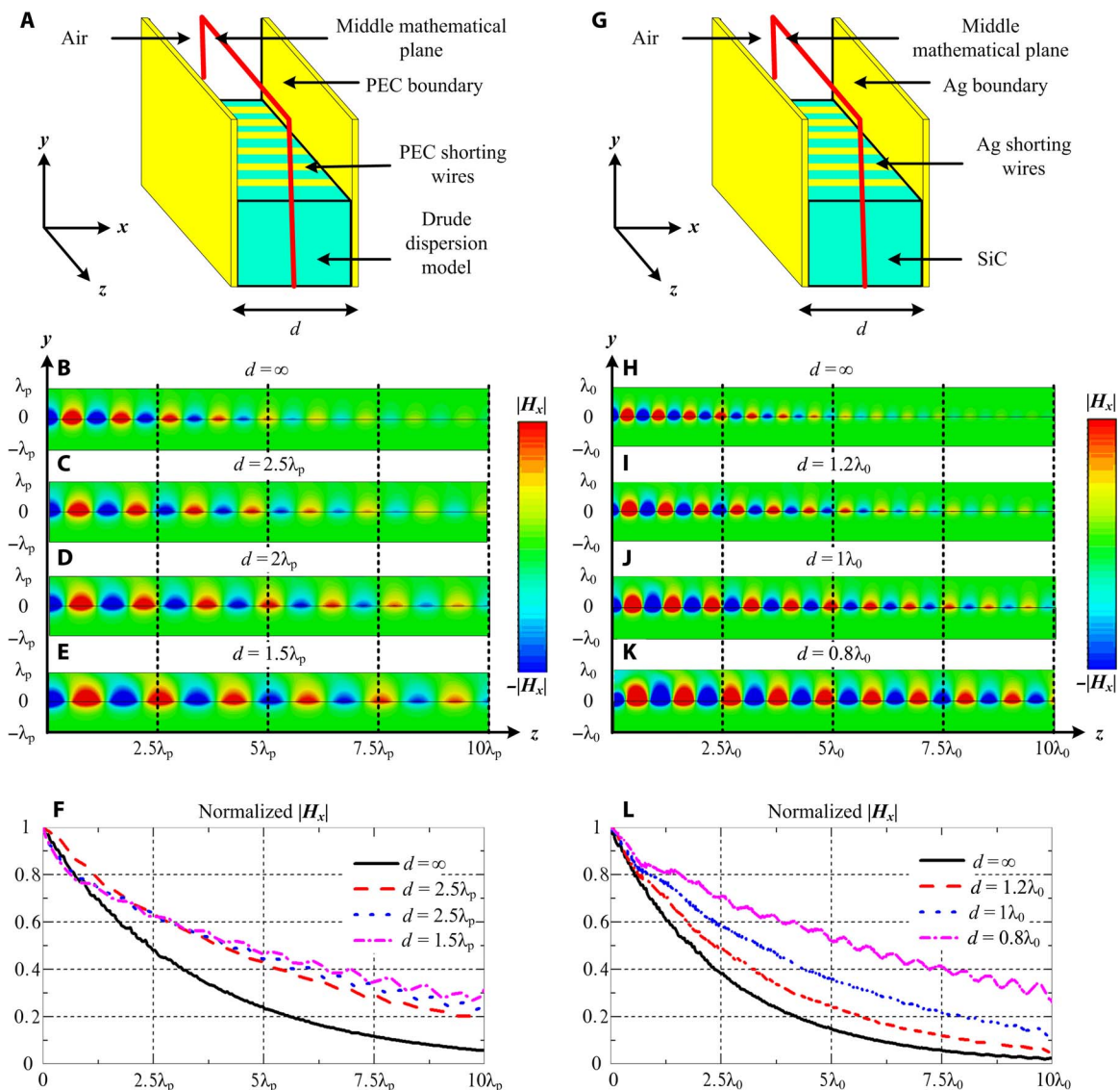
Fig. 5. Field distributions for structural-based SPP propagation. (A) Lossy plasmonic materials using the Drude model with \gamma = 0.03\omega_p , bounded by PEC PPW with the width of d . The overall length is 10\lambda_p along the z axis. Snapshots of H_x distributions in the middle mathematical plane at \omega = 0.6\omega_p : (B) d = \infty (i.e., with no parallel plates), (C) d = 2.5\lambda_p , (D) d = 2\lambda_p , and (E) d = 1.5\lambda_p . (F) Normalized magnitude of H_x along the z axis. (G) Practical scenario: SiC using the Lorentzian model in Eq. 9, bounded by Ag using the Drude model in Eq. 10, with the width of d and the thickness of \lambda_0/5 , \lambda_0 = 10.7 \mu\text{m} at 28 THz. The overall length is 10\lambda_0 in the z direction. Snapshots of H_x distributions in the middle mathematical plane at 28 THz: (H) d = \infty (i.e., with no parallel plates), (I) d = 1.2\lambda_0 , (J) d = 1\lambda_0 , and (K) d = 0.8\lambda_0 . (L) Normalized magnitude of H_x along the z axis.
