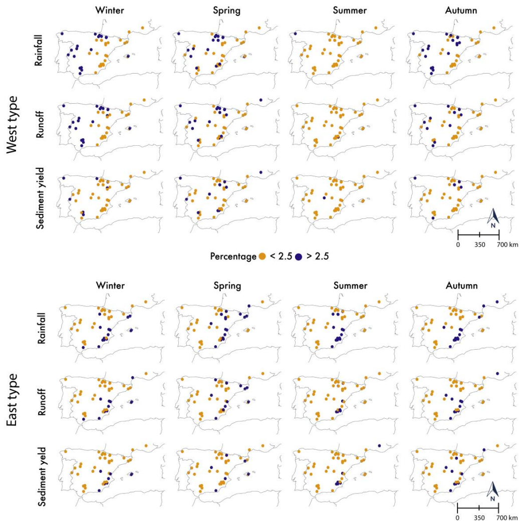
Figure 4. Spatial distribution of the percentage of rainfall, runoff and sediment yield in the west (W) and east (E) weather types for each season. The 2.5% value represents the uniform distribution of 10 WTs and 4 seasons.
