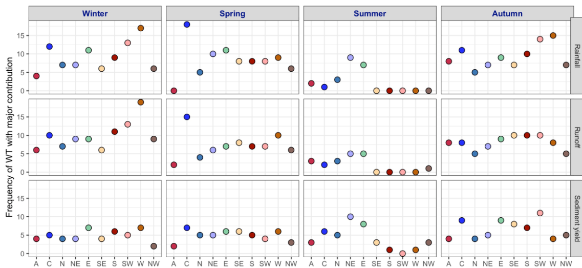
Figure 6. Frequency of the weather types with the major contribution (more than 5%) of the percentage of rainfall, runoff, and sediment yield in each season.
