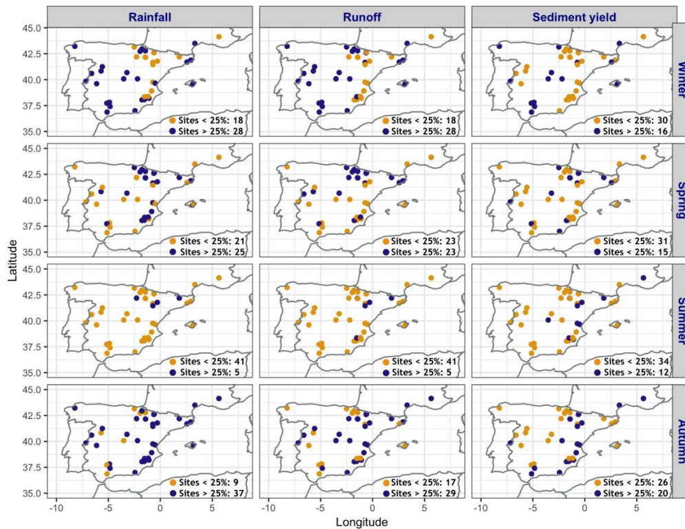
Figure 2. Spatial distribution of the percentage of rainfall, runoff, and sediment yield for each season in the study sites, and the number of sites with values higher or lower than 25%.
