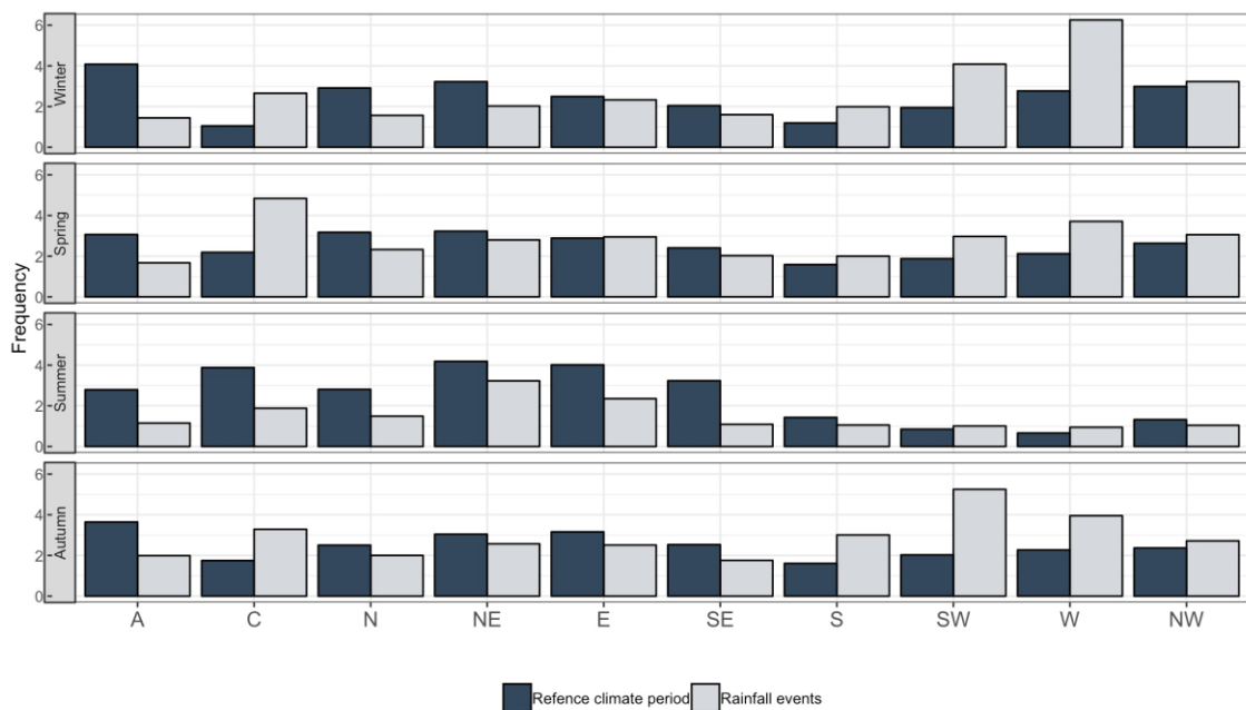
Figure 5. Frequency of the reference climate period (1981–2010) and in the study events (1985–2015) in the WTs in each season.
