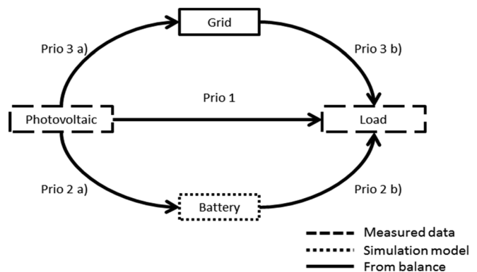
FIG. 4. Conceptual flow diagram of the dispatching model used for the simulation of the investigated district.
