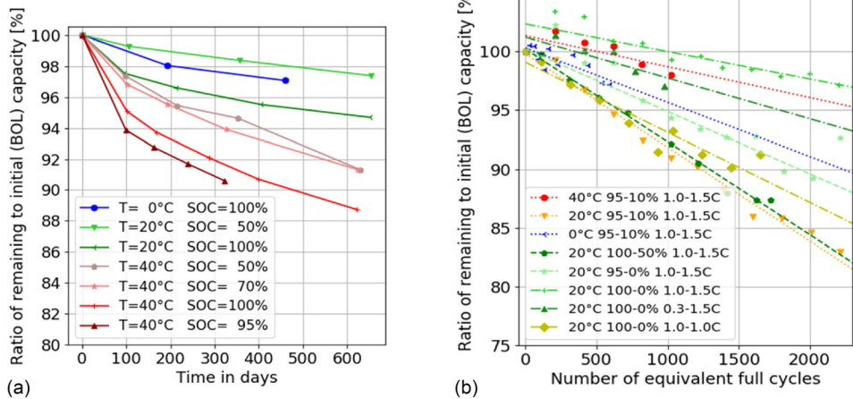
FIG. 16. Experimental results for the degradation tests including calendric and cycle aging for the LFP lithium-ion reference battery cell.
