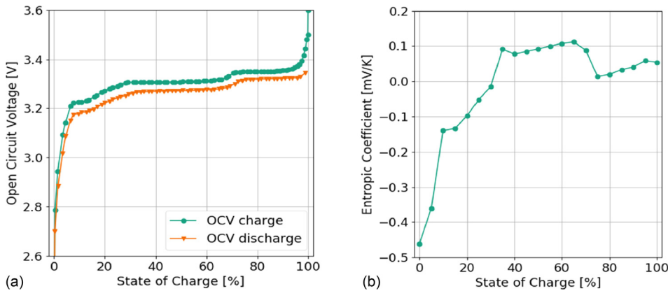
FIG. 14. Experimental results for the open-circuit and entropic coefficient results, as a function of the state-of-charge, obtained for the LFP lithium-ion reference battery cell.
