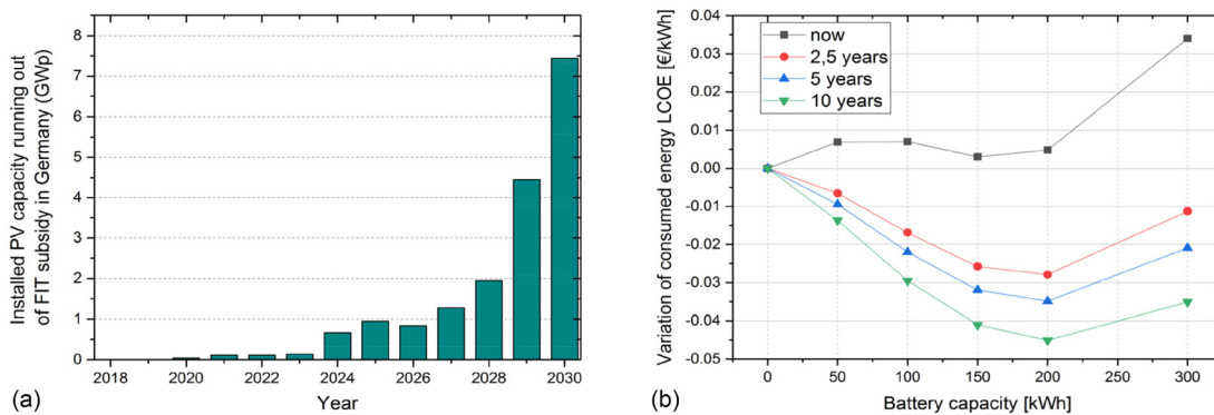
FIG. 13. Upcoming scenario for battery retrofitting of the existing PV system: (a) Prognosis of PV installed capacity, in Germany, which will finish receiving the FIT subsidy. (b) Variation of PV battery LCOE as a function of the installed battery capacity in PV installations for which the FIT subsidy has prescribed.
