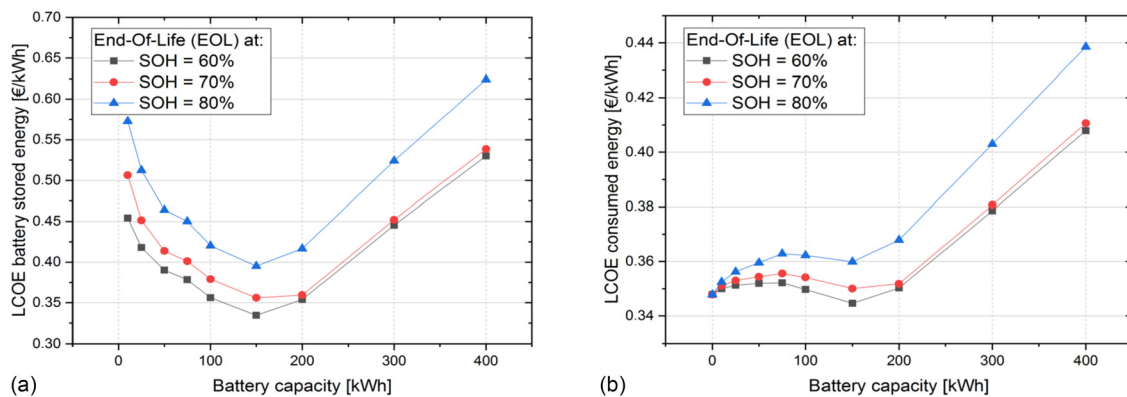
FIG. 11. Effects of battery end-of-life (EOL) criteria on (a) LCOE of the stored energy and (b) LCOE of the consumed energy. These results are obtained for a PV capacity of 150 kWp.
