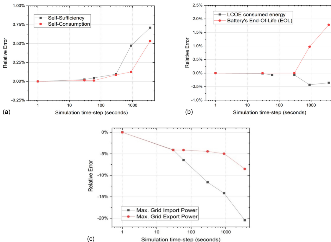
FIG. 6. Time-step convergence. Plot of the relative error from representative model variables, as compared with the results obtained with 1-s granularity. The results are shown for (a) the self-sufficiency and self-consumption indicators; (b) the LCOE and battery life predictions; (c) the maximum grid import and export power flows.
