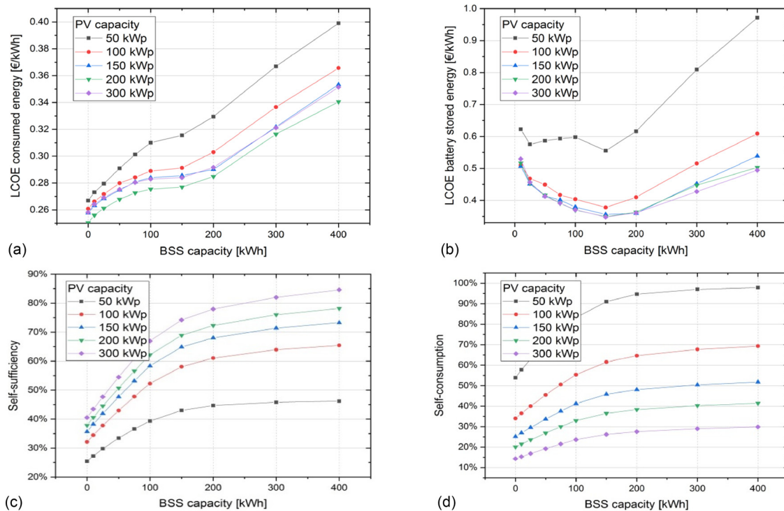
FIG. 9. Effects of battery installed capacity, in kWh, on the levelized cost of consumed and stored energy and on the self-sufficiency and self-consumption indexes.
