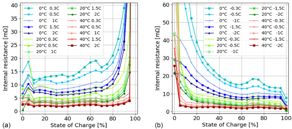
FIG. 15. Experimental results for the internal resistance, as a function of the state-of-charge, the temperature, and the current rate, obtained for the LFP lithium-ion reference battery cell.
