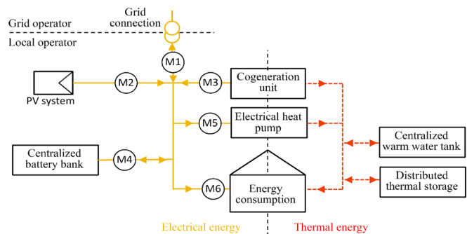
FIG. 2. Scheme of the power and heat supply system and installed electrical metering points (M1 to M6) at the case study district in Weinsberg.
