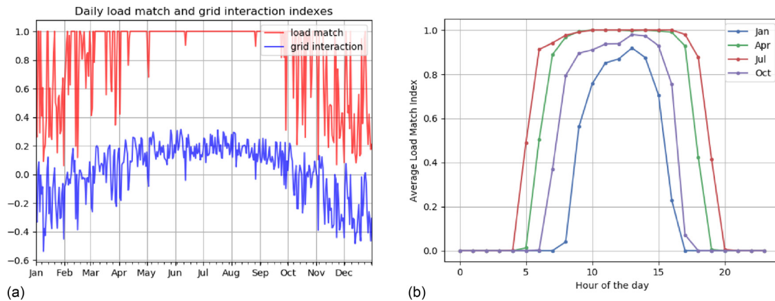
FIG. 19. Left figure (a) shows obtained daily load match and grid interaction indexes throughout one year. On the right (b), average hourly load match indexes are plotted for 4 representative months. The results shown have been obtained with a 200 kWp PV, 200 kWh battery system.
