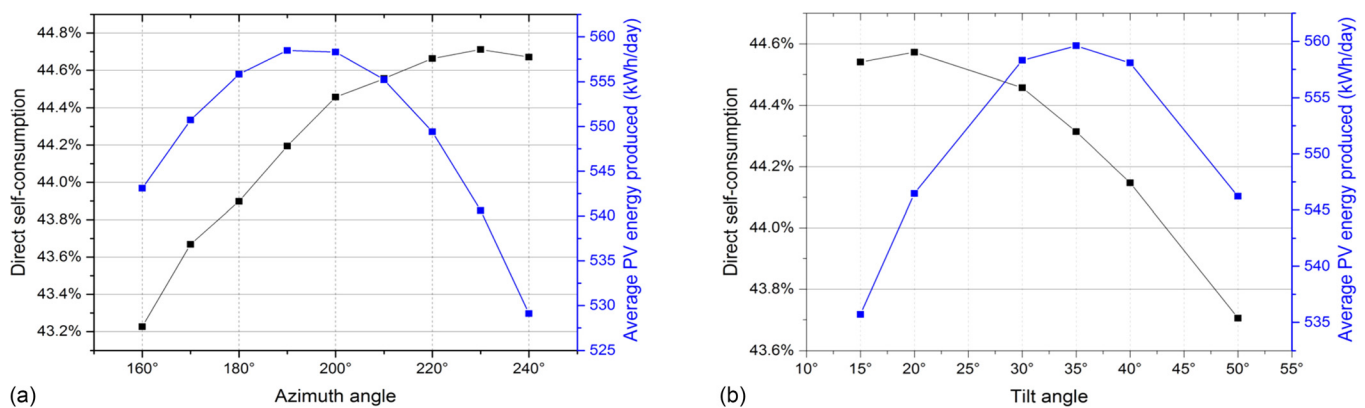
FIG. 7. Self-consumption and PV energy production as functions of (a) azimuth angle and (b) tilt angle. These results were obtained with a PV installed capacity of 200% the maximum load.
