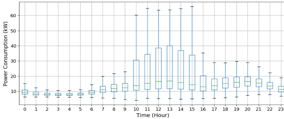
FIG. 3. Boxplot of the average electrical power consumption distribution throughout the hour of the day. In this plot, the boxes show the quartiles Q1, median (Q2), and Q3 of the data, while whiskers are limited by extreme data measurements or 1.5 times the interquartile range (IQR).
