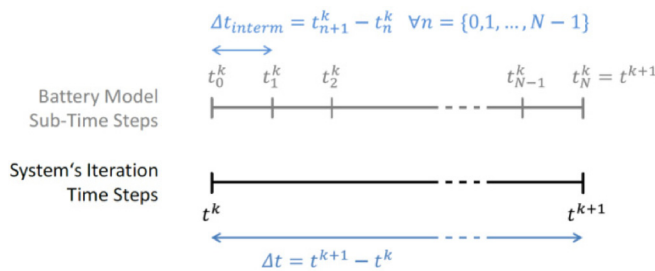
FIG. 18. Iterative scheme employed for the time-integration of battery model performance.
