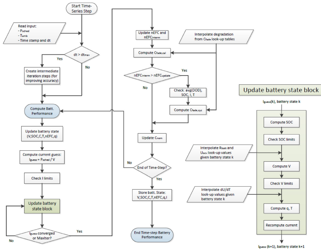
FIG. 17. Flowchart of the implemented battery model.
