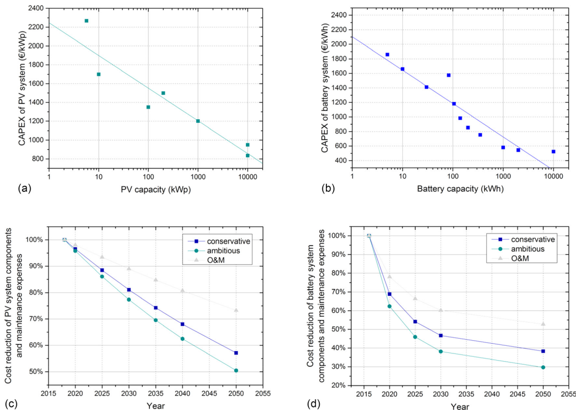
FIG. 5. Cost of PV and battery: (a) and (b) as a function of component size and (c) and (d) as a function of the installation year.
