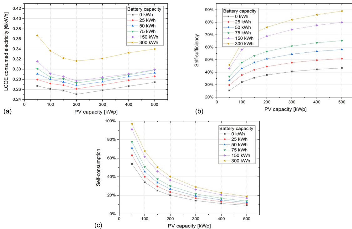
FIG. 8. Effects of PV installed capacity, in kWp, (a) on the levelized cost of consumed energy, (b) on the self-sufficiency, and (c) on the self-consumption indexes.
