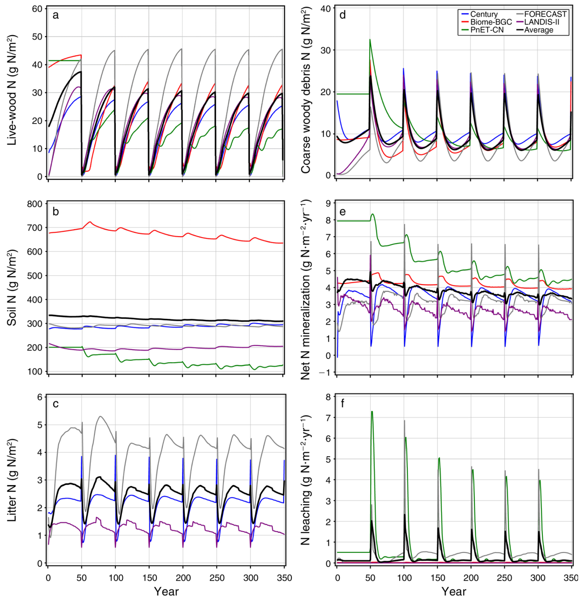
FIG. 3. Nitrogen pools and fluxes and CN interaction of an aspen forest ecosystem on glacial outwash plains in Wisconsin disturbed by bole-only harvesting every 50 yr. Colored lines represent the results of simulations of the five models Biome-BGC, CENTURY, FORECAST, LANDIS-II-Century, and PnET-CN. The black line is the average of all models.
