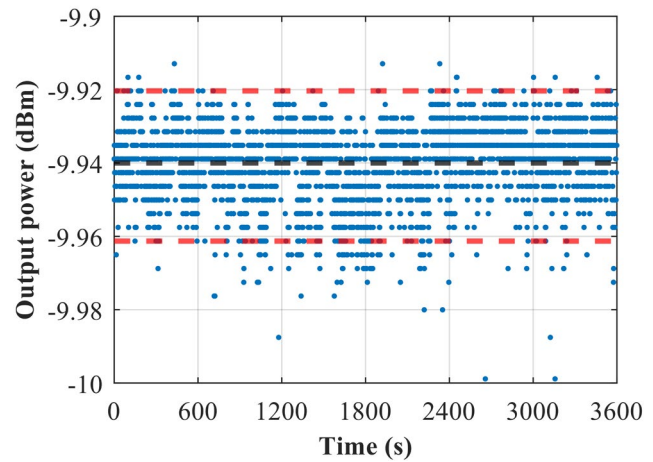
Fig. 7. Output power stability when pumped by a 976-nm laser at 100 mW and using the ACBFR, measured over 1 h with a CL of 95 %. The red dashed lines represent the confidence interval limits, while in black the mean peak power is plotted.
