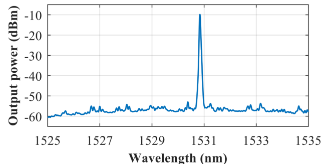
Fig. 4. Output spectra of the ring-cavity fiber laser when pumped by a 976-nm laser at 100mW while using the ACBFR, measured by an OSA.
