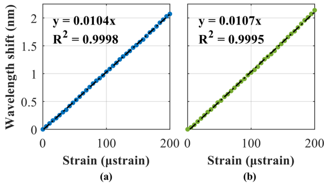
Fig. 13. Wavelength shift as function of the strain applied to the ACBFR for the C-band laser (a), and L-band laser (b).
