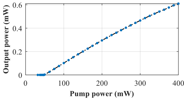
Fig. 5. Output power versus pump power for the C-band ACBFR-based fiber laser.
