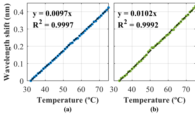
Fig. 12. Wavelength shift as function of temperature when using the ACBFR for the C-band laser (a), and L-band laser (b).
