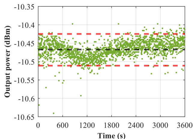
Fig. 11. Output power stability of the L-band laser when pumped at 100 mW while using the ACBFR, measured over 1 h with a CL of 95 %. Red dashed lines represent the confidence interval limits. The mean peak power is plotted in black.
