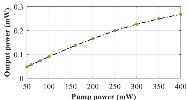
Fig. 9. Output power versus pump power for the L-band ACBFR-based fiber laser.
