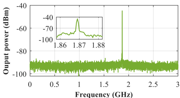
Fig. 10. Output spectra of the L-band ring-cavity fiber laser when pumped at 100 mW while using the ACBFR, measured by an ESA when a TLS was tuned close to 1598.8 nm.
