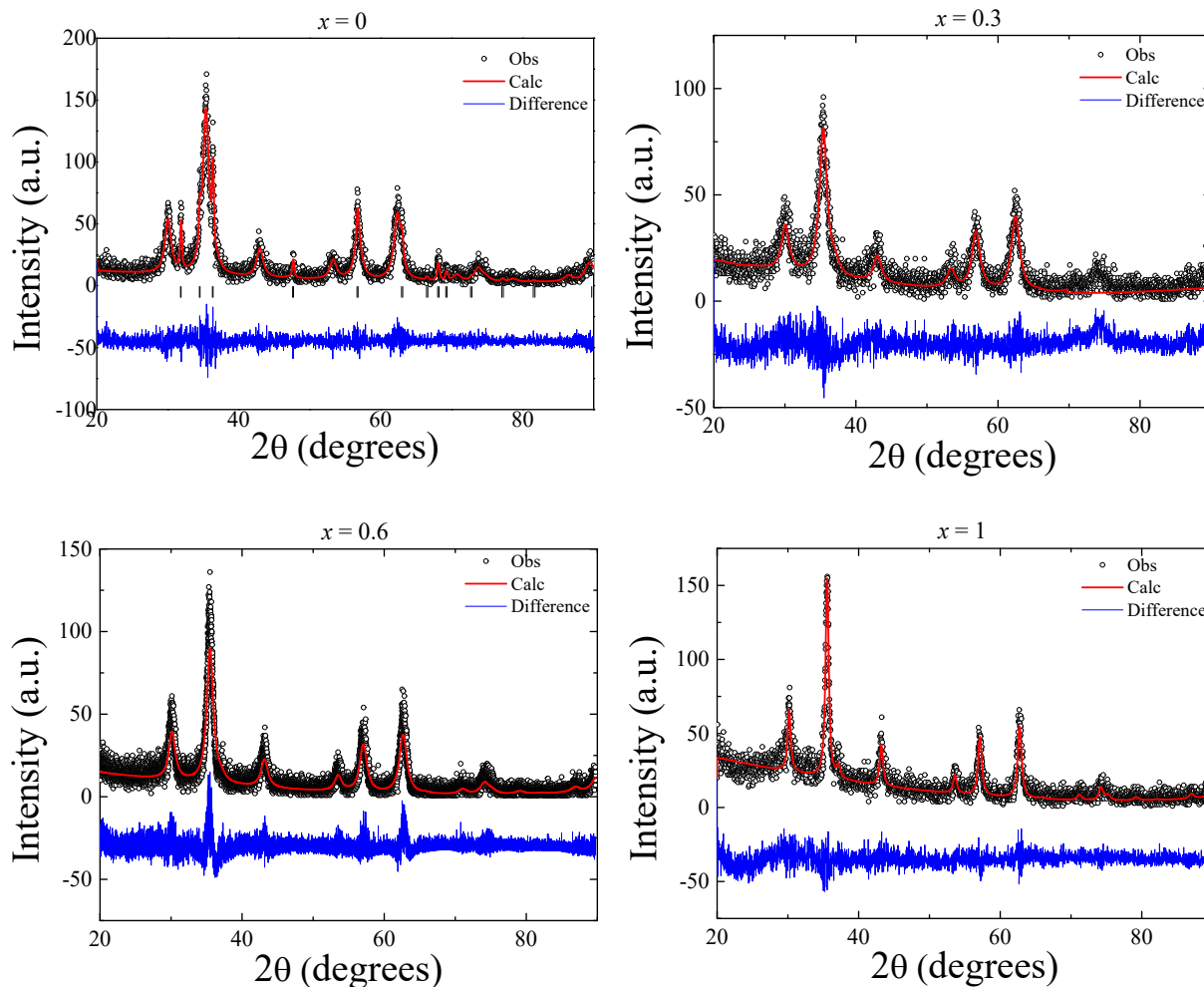
Fig. 1. XRD Rietveld adjustments for \text{Co}_x\text{Zn}_{1-x}\text{Fe}_2\text{O}_4 nanoparticles ( x = 0, 0.3, 0.6 and 1) (o) experimental and (—) calculated intensities. The difference between both intensities is shown at the bottom of the figures (—). The Bragg reflections of ZnO are shown (|).
