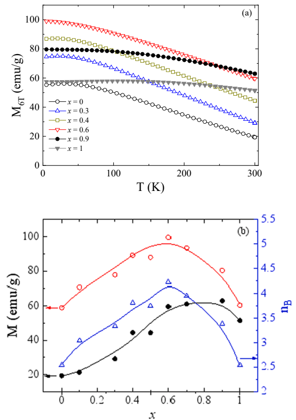
Fig. 7. (a) Temperature dependence of the high field magnetization ( M_{6T} ) for the \text{Co}_x\text{Zn}_{1-x}\text{Fe}_2\text{O}_4 nanoparticles ( \mu_0H = 6 T); (b) (○) saturation magnetization, M_0 , obtained from the Bloch's law; (△) the number of Bohr magnetons, n_B , per formula unit and (●) the experimental high field magnetization ( \mu_0H = 6 T) at 300 K.
