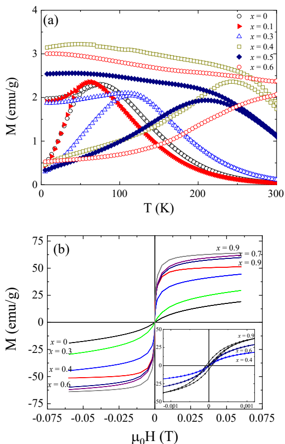
Fig. 8. (a) ZFC-FC magnetization curves (50 Oe) and (b) Room temperature hysteresis loops for the indicated \text{Co}_x\text{Zn}_{1-x}\text{Fe}_2\text{O}_4 nanoparticles. Inset: enlargement of the low field region.
