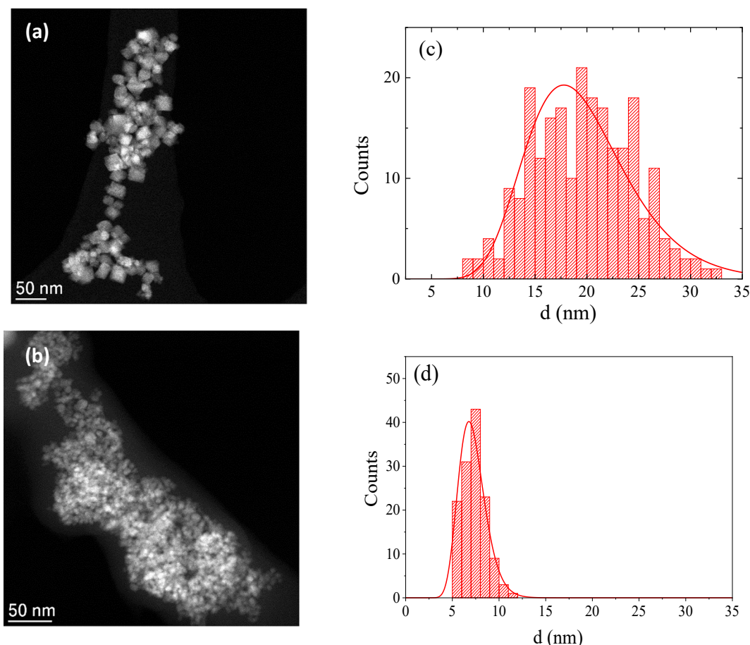
Fig. 2. STEM images (a) and (b) of \text{Co}_x\text{Zn}_{1-x}\text{Fe}_2\text{O}_4 nanoparticles x = 1 , x = 0.3 , respectively; (c) x = 1 and (d) x = 0.3 nanoparticle size ( d : diameter) distribution.
