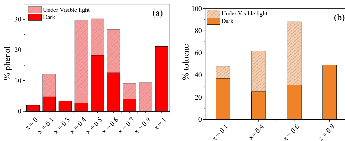
Fig. 9. (a) Phenol photodegradation (% phenol) and (b) Toluene photodegradation (% toluene) in the presence of \text{Co}_x\text{Zn}_{1-x}\text{Fe}_2\text{O}_4 nanoparticles under dark (solid bars) and under radiation (striped bars).
