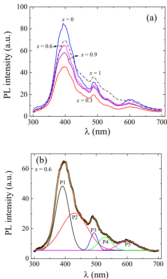
Fig. 6. Photoluminescence spectra for \text{Co}_x\text{Zn}_{1-x}\text{Fe}_2\text{O}_4 : (a) x = 0, 0.3, 0.6, 0.9, 1 ; (b) deconvoluted PL peaks for x = 0.6 .
