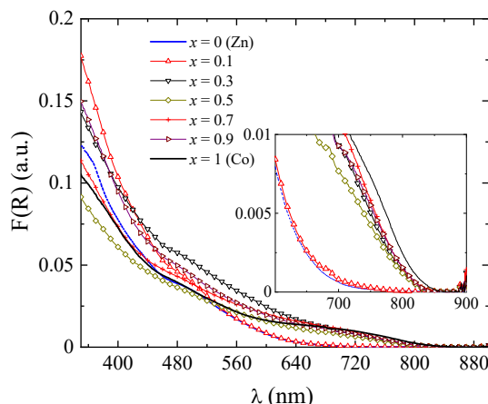
Fig. 4. UV-Vis absorption curves obtained from the Diffuse Reflectance Spectroscopy (DRS) for some selected \text{Co}_x\text{Zn}_{1-x}\text{Fe}_2\text{O}_4 nanoparticles.
