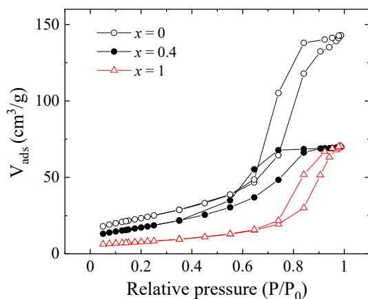
Fig. 3. Nitrogen adsorption-desorption curves at 77 K for \text{Co}_x\text{Zn}_{1-x}\text{Fe}_2\text{O}_4 nanoparticles.
