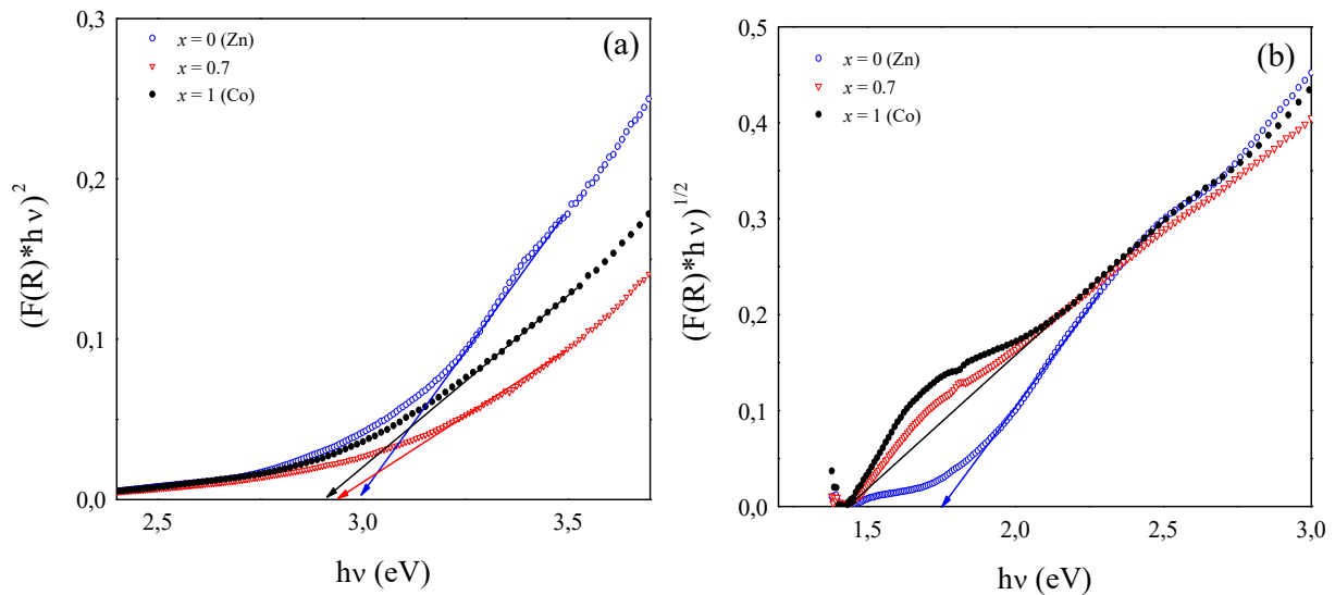
Fig. 5. Tauc plots of (a) direct and (b) indirect band gap for some selected \text{Co}_x\text{Zn}_{1-x}\text{Fe}_2\text{O}_4 nanoparticles.
