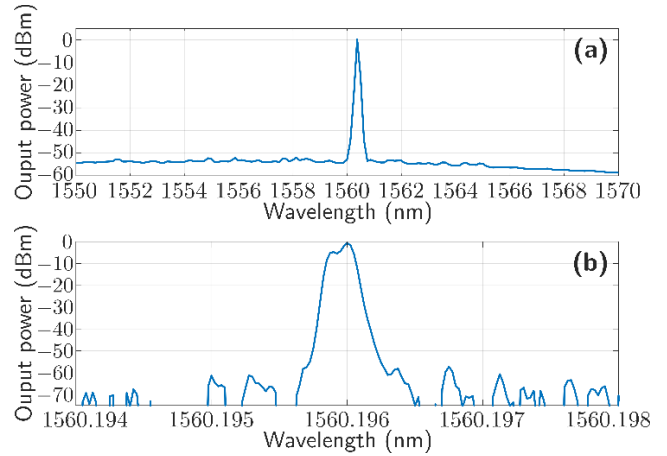
FIGURE 5. Output optical spectrum of the linear-cavity fiber laser with MD-EDF pumped by a 976nm laser at power of 100mW without using the optical variable attenuator, measured by the OSA (a) and the BOSA (b).
