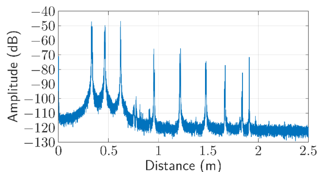
FIGURE 2. Backscattered optical power as a function of fiber length for a 2-meters-long micro-drilled erbium-doped fiber section.
