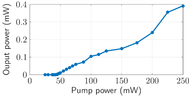
FIGURE 4. Output power versus pump power for the linear cavity fiber laser.
