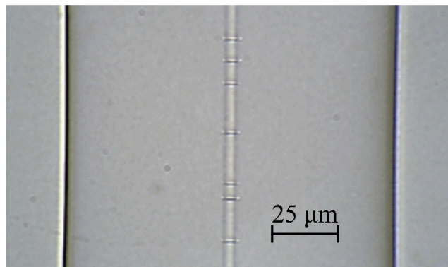
FIGURE 1. Microscope image of one of the nine quasi-randomly distributed reflectors inscribed along the erbium doped fiber.
