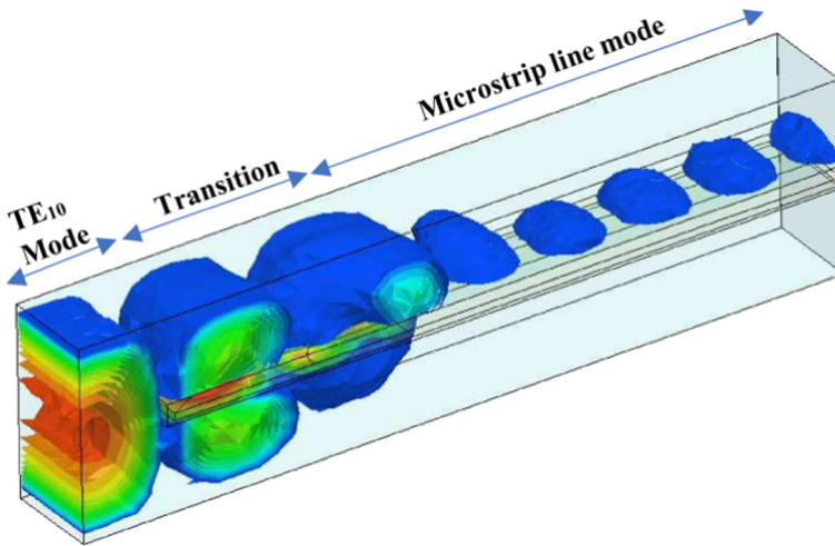
Fig. 4 E-field distribution at 0.305 THz. The TE_{10} mode entering the transition from left is split, rotated and finally matched to the microstrip quasi-TEM mode
