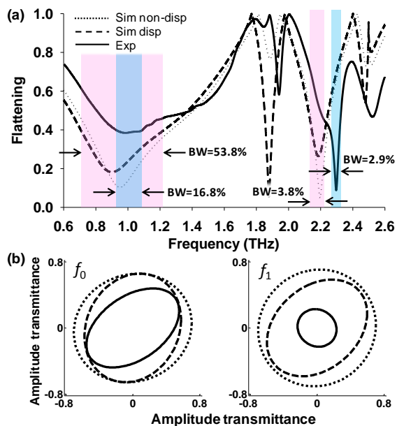
Fig. 3. (a) Flattening of the polarization state for the transmitted wave. Shaded areas represent the operational bandwidths. (b) Polarization state at the optimum frequencies.
