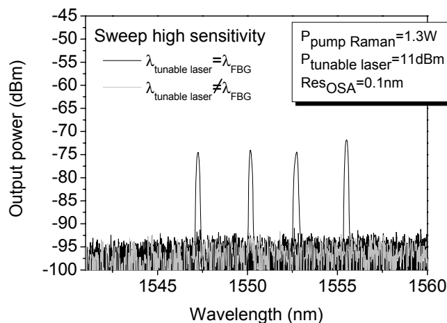
Figure 9. Spectrum of the reflected signal from the four FBG using OSA option sweep high sensitivity.
