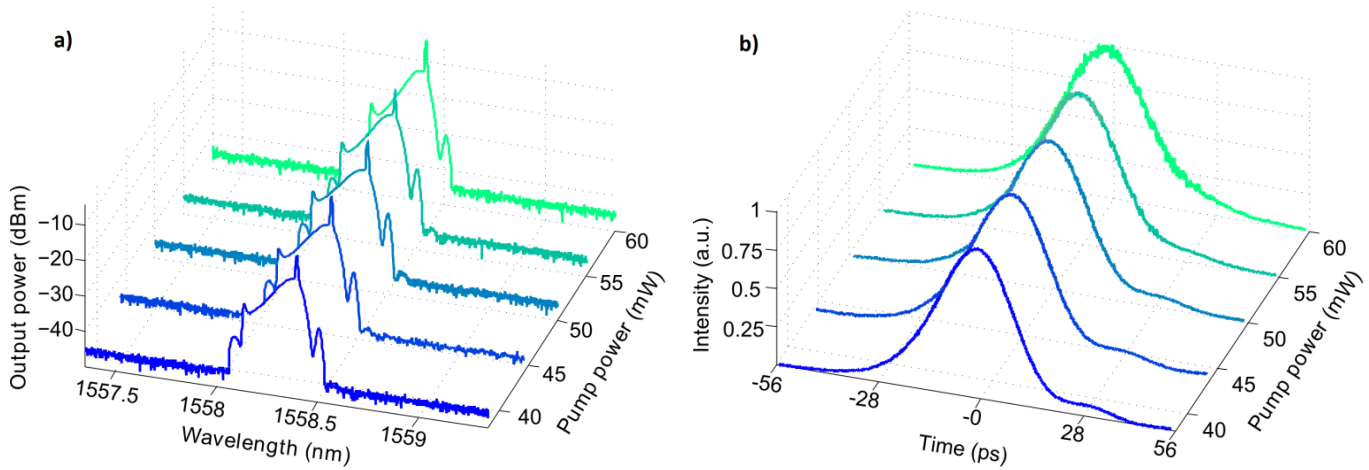
Fig.4 a) Optical output spectra and b) temporal traces of the ML soliton centered at 1558.4 nm for different pump powers
