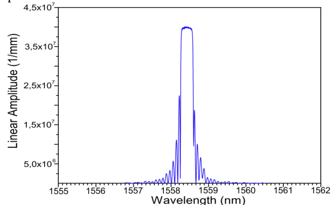
Fig.2 Optical spectrum of the saturated FBG
