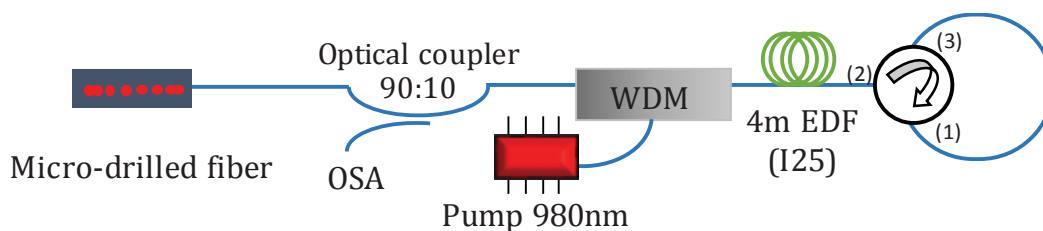
Figure 2. Schematic diagram of the experimental linear short-cavity fiber laser setup, in which the micro-perforated fiber was used to reflect an amplified signal.
