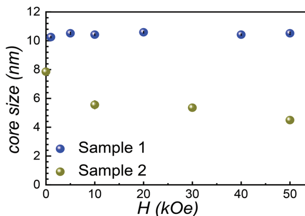
Figure 5. Dependence of the core size of the \text{Fe}_3\text{O}_4 counterpart of samples 1 and 2 on the applied magnetic field. The error bars (about \pm 0.5 nm for sample 1 and \pm 2 nm for sample 2), that is, estimates standard deviation from the CrysPy refinement, do not exceed the symbol size.
