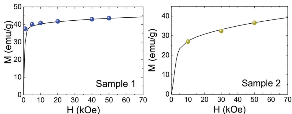
Figure 7. Initial magnetization (solid line; measured by SQUID) and the averaged total magnetic moment (symbols; obtained from the CrysPy refinement \times 0.4 ) for the samples 1 (left) and 2 (right). The error bars, that is, estimates standard deviation from the CrysPy refinement, do not exceed the symbol size.
