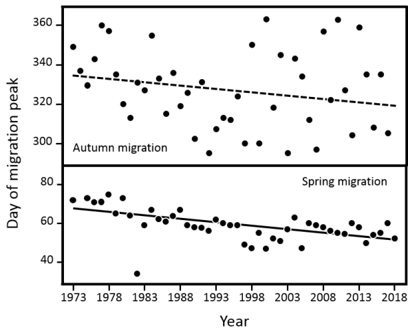
Fig. 5. Date of maximum number of Common Cranes ( Grus grus ) in autumn (top) and spring (bottom) migrations. Common Cranes advanced the migration in spring 16.2 days ( P < 0.001 ) but not in autumn ( P > 0.05 ). Lines show linear regression fits, respectively statistically significant (continuous line) and nonsignificant (dashed line).
