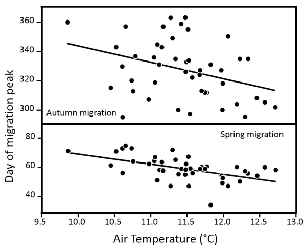
Fig. 6. Dates of migratory peaks in autumn (top) and spring (bottom) advanced with higher annual mean temperatures. Linear regression fits were statistically significant in autumn ( P < 0.05 ) and spring ( P < 0.01 ): on average, Common Cranes ( Grus grus ) significantly advanced their migration time by 10.4 days in autumn and 11.6 days in spring per ^{\circ}\text{C} increase.
