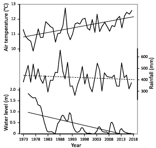
Fig. 1. Mean annual air temperature (top), annual precipitation (middle), and water level of the lagoon (bottom) in Gallocanta between 1973 and 2018. Temporal trends (highlighted with linear regression fitting lines) are statistically significant ( P < 0.001 ) for air temperature increase and water level decrease (continuous lines). Annual precipitation did not show a significant temporal trend (dashed line).
