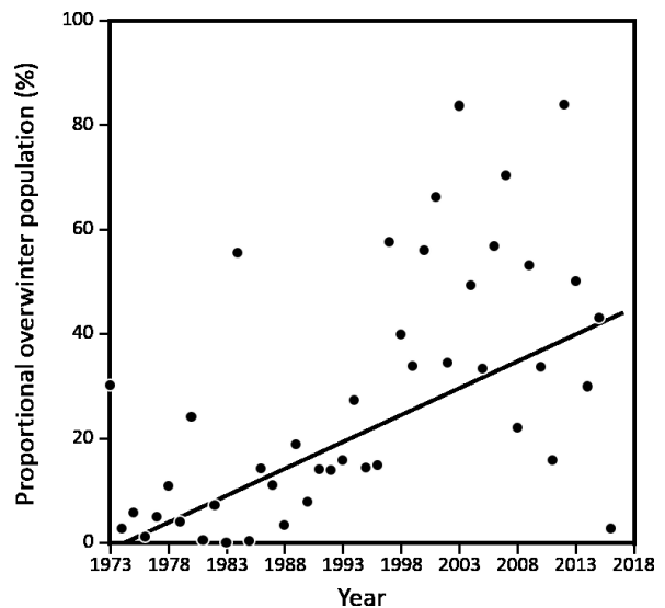
Fig. 4. Ratio of the minimum number of Common Cranes ( Grus grus ) in winter to the maximum number of Common Cranes during autumn migration throughout the study period. The continuous line shows a linear regression fit ( P < 0.001 ).
