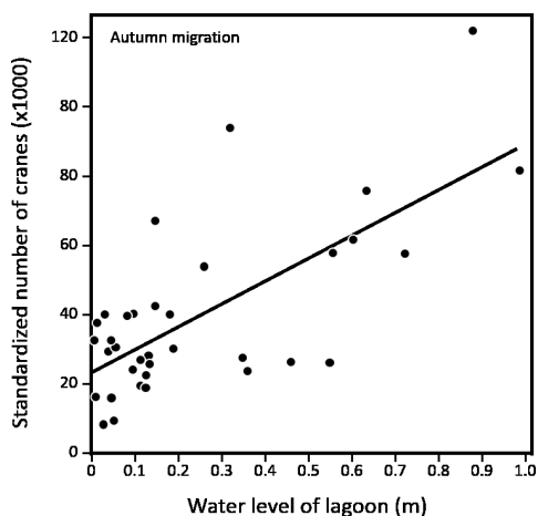
Fig. 3. Relationship between the maximum number of Common Cranes ( Grus grus ) in autumn migration (period 1983 to 2018) and the annual mean of water level. Numbers of Common Cranes were previously standardized to the autumn peak of year 2018 to control for the population increase along the study (see Methods). The line shows a linear regression fit ( P < 0.001 ).
