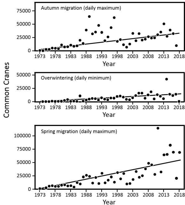
Fig. 2. Maximum numbers of Common Cranes ( Grus grus ) counted in Gallocanta during the autumn (top) and spring (bottom) migration periods, and minimum number during the overwintering period (middle). Temporal trends (highlighted with linear regression fitting lines) are all statistically significant ( P < 0.001 ).
