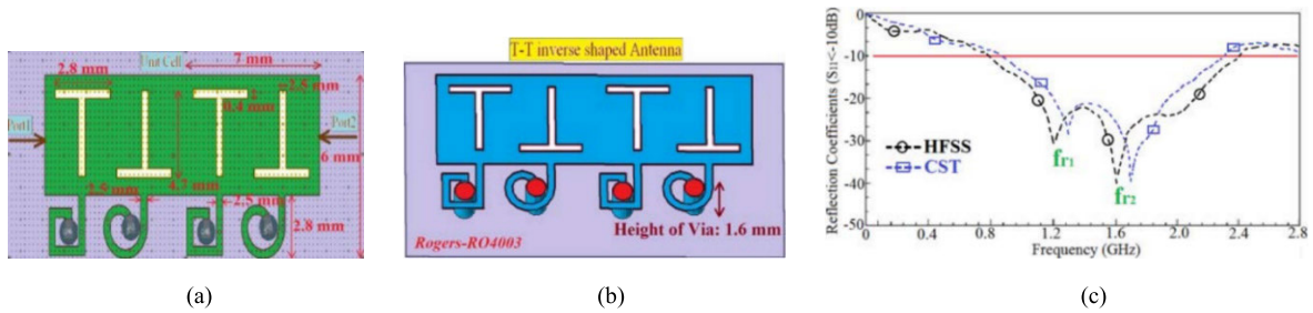
FIGURE 25. Antenna, and its reflection coefficient responses [41].
