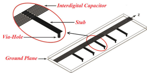
FIGURE 6. 1-D microstrip CRLH TL constructed of interdigital capacitors and shorted-stub inductors [11].
