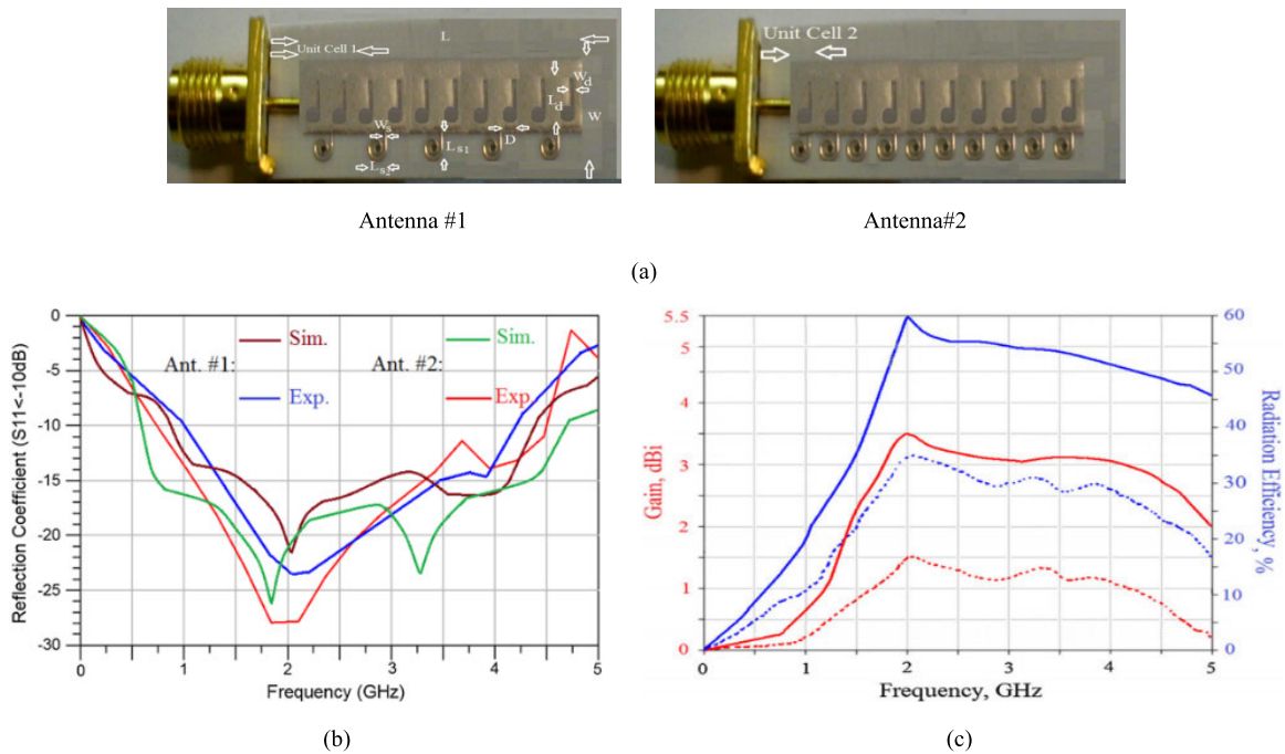
FIGURE 20. (a) Two planar slotted antennas, (b) reflection-coefficient responses, (c) gain and efficiency performances. (Ant.#1: Dashed-lines, and Ant.#2: Solid-lines) [36].
