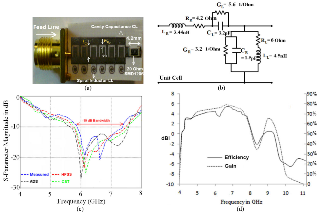
FIGURE 24. (a) MTM antenna, (b) unit-cell’s circuit model, (c) reflection-coefficients, and (d) gain and radiation efficiency [40].
