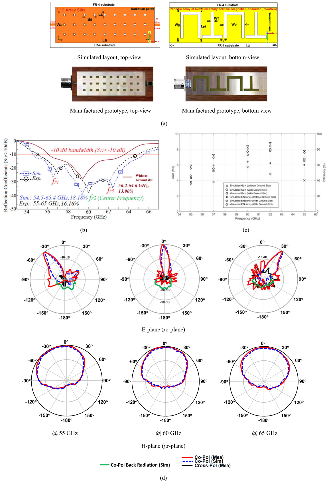
FIGURE 13. (a) Leaky-wave antenna, (b) reflection coefficient responses before and after implement the GND slots. Dashed lines plot the case after apply the slots, (c) radiation gain and efficiency responses when the antenna has unloaded and loaded with GND slots, and (d) backward to forward radiation patterns [31].
