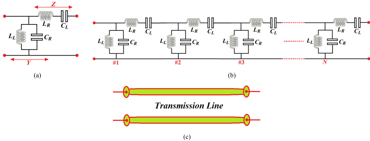
FIGURE 5. LC-based CRLH TL. (a) Unit-cell. (b) LC periodic network, and (c) homogeneous CRLH TL, which is equivalent to (b).
