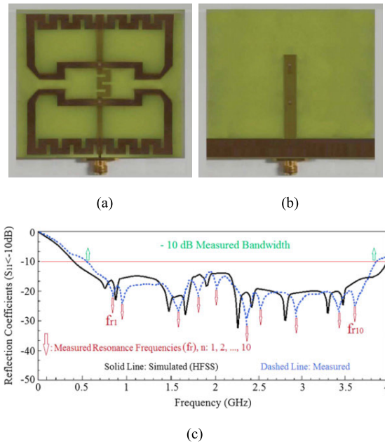
FIGURE 9. Proposed meandered antenna, (a) top surface, (b) back-side, and (c) reflection coefficients [53].
