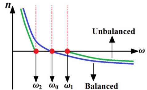
FIGURE 4. Typical index of refraction diagrams for the balanced- and unbalanced-CRLH TLs in blue and green, respectively.
