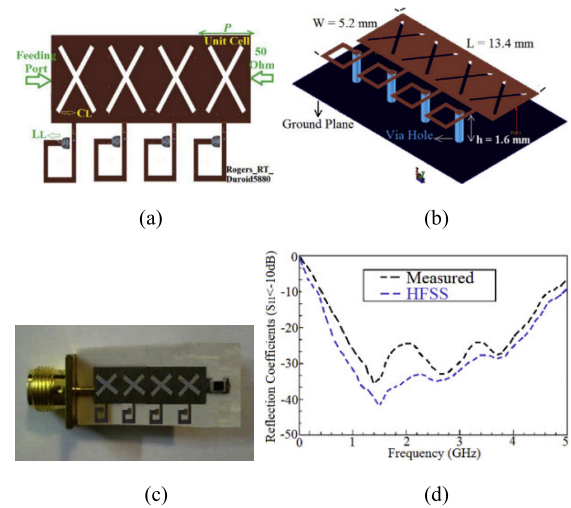
FIGURE 16. (a-c) Antenna's layout, and (d) its reflection coefficients responses [46].
