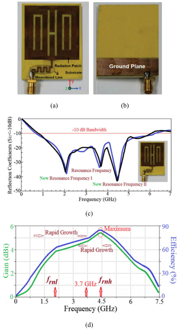
FIGURE 10. (a) Top surface of the proposed antenna, (b) its bottom side, (c) its reflection coefficient, and (d) its radiation gain and efficiency curves [54].
