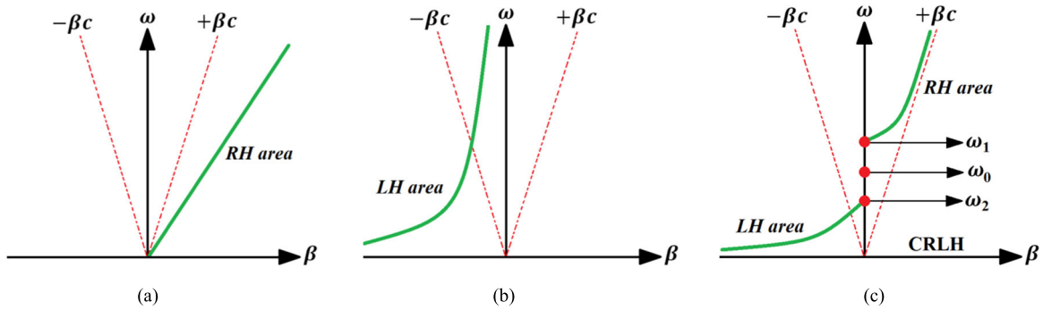
FIGURE 2. Dispersion curves for the transmission lines of the Fig.1. (a) RH transmission line, (b) LH transmission line, and (c) CRLH transmission line (unbalanced).
