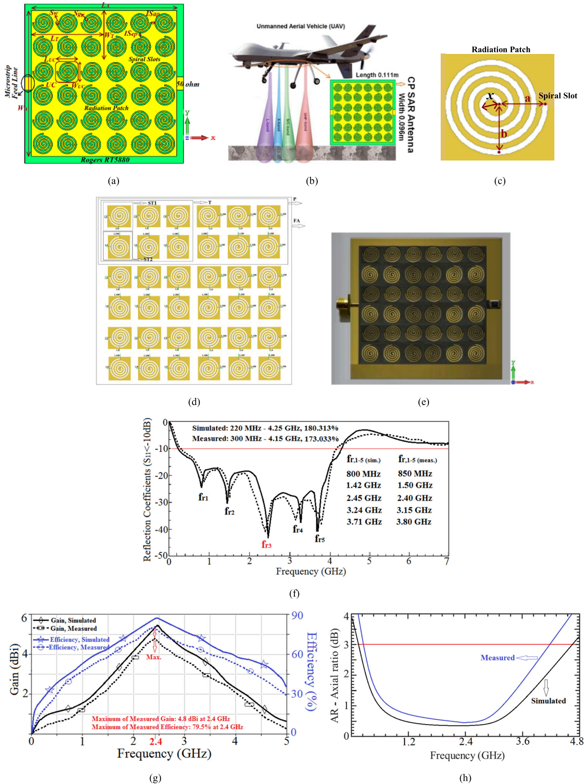
FIGURE 30. (a) Array antenna with direct feed-line, (b) Array antenna onboard a UAV, (c) radiating unit-cell element, (d) applied cross-polarization suppression methods. (e) Photograph of the SAR array antenna, (f) reflection coefficient responses, (g) Gain and radiation efficiency, and (h) Axial-ratio at \theta = 0^\circ [48].
