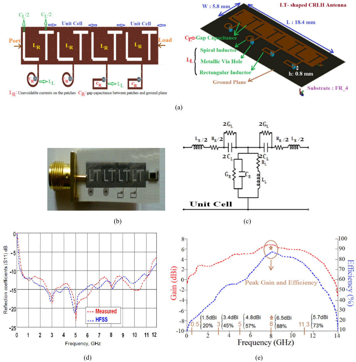
FIGURE 22. (a) CRLH antenna, (b) its manufactured prototype, (c) unit cell' circuit model, (d) reflection coefficients, and (e) radiation gain and efficiency [38].
