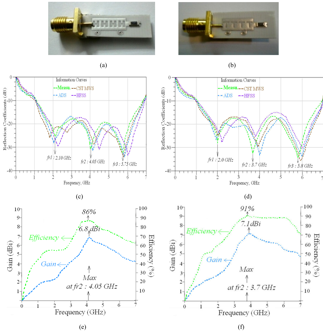
FIGURE 26. (a) H-antenna, (b) T-antenna, (c) H-antenna's reflection-coefficient responses, (d) T-antenna's reflection-coefficient responses, (e) H-antenna's gain and radiation efficiency responses, and (f) T-antenna's gain and radiation efficiency response[42].
