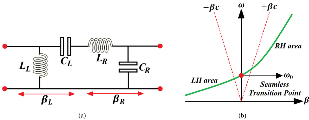
FIGURE 3. Balanced case of the Fig.1(c). (a) simplified circuit model, and (b) dispersion curve displaying seamless LH to RH transition.
