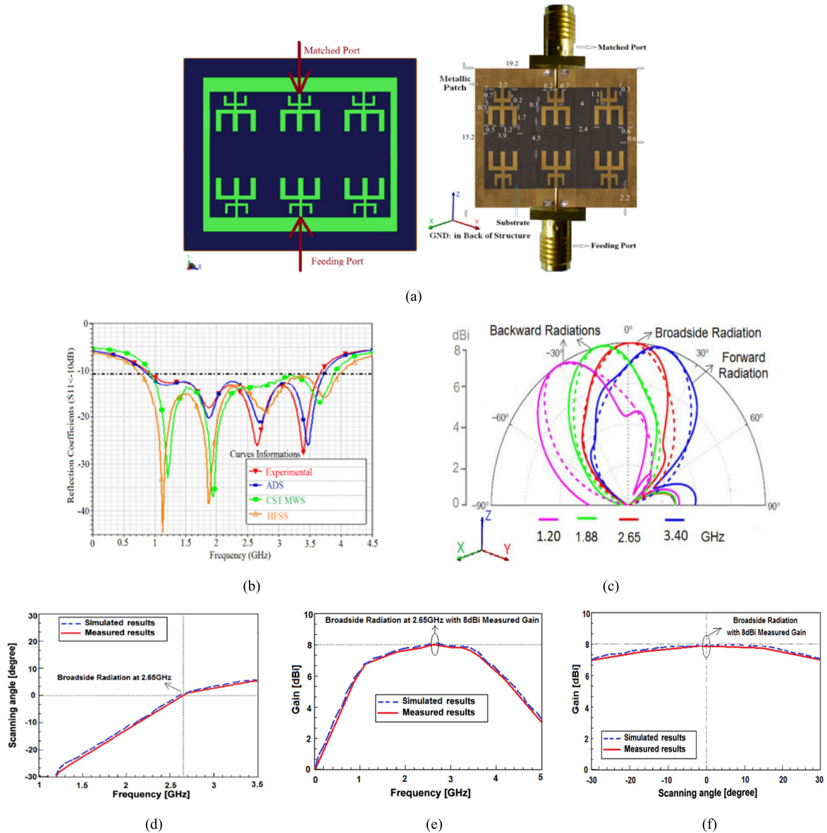
FIGURE 14. (a) Prototypes of the LWA (structural parameters have mentioned in millimeter), (b) reflection coefficients, (c) 2-D radiation patterns. Solid and dashed lines represents the measured and simulated results, respectively, (d) Scanning angle as function of the frequency, (e) Gains curves as function of the frequency, and (f) Gain curves versus scanning angle [32].
