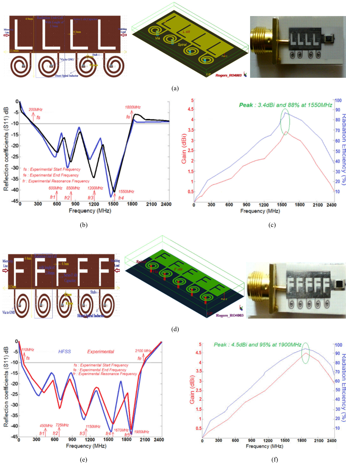
FIGURE 28. (a) L-shaped antenna, (b) its reflection coefficient responses, (c) its radiation gain and efficiency, (d) F-shaped antenna, (e) its reflection coefficients responses, and (f) its radiation gain and efficiency [44].
