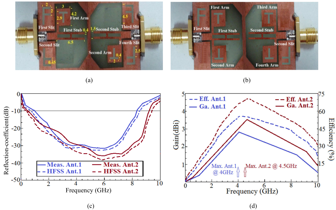
FIGURE 31. (a) Antenna #1, (b) Antenna #2, (c) reflection-coefficient responses, and (d) measured gain and radiation efficiency responses [49].
