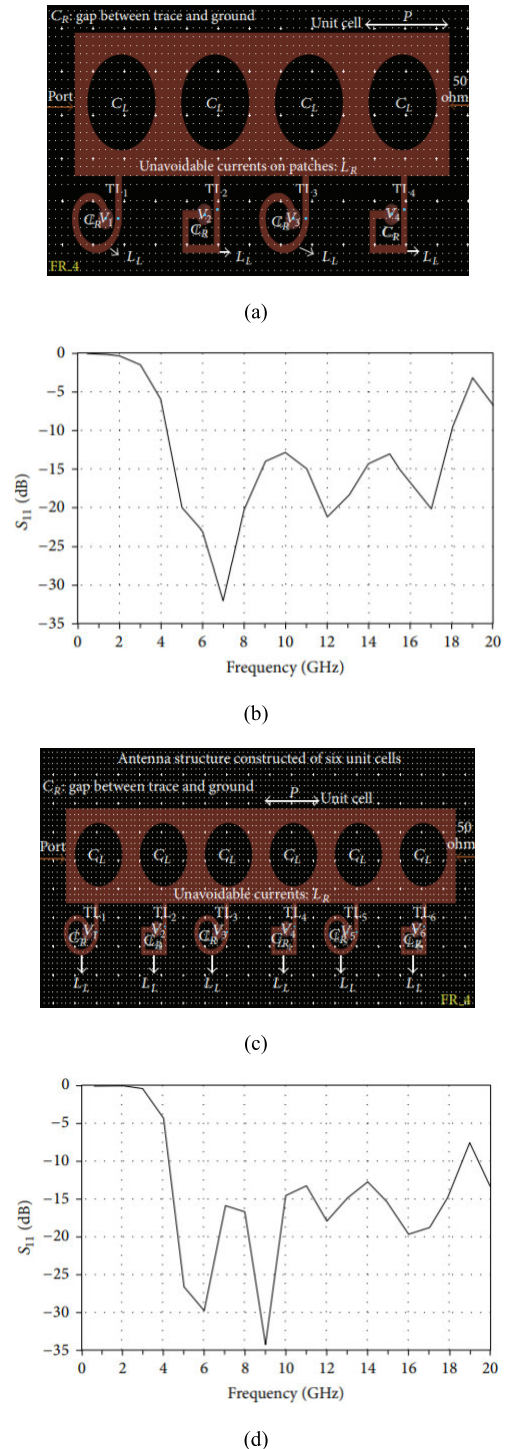
FIGURE 11. (a) Metamaterial-TL based antenna with four cells, (b) its reflection coefficient, (c) MTM-TL based antenna constructed of six-cells, (d) its reflection coefficient [55].
