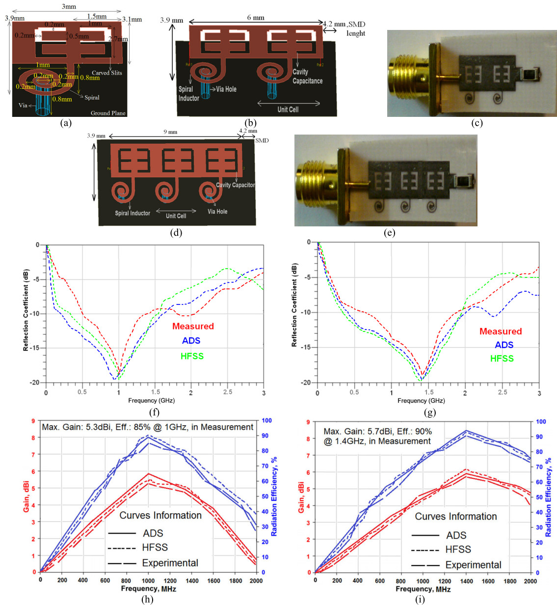
FIGURE 17. (a) Proposed unit cell layout of the resonating MTM based miniaturized antennas, (b, c) E-formed antenna constructed of two cells, (d, e) E-formed antenna constructed of three cells, (f, g) reflection coefficients responses for first and second antennas, respectively, (h, i) gain and radiation efficiency curves for first and second antennas [78].
