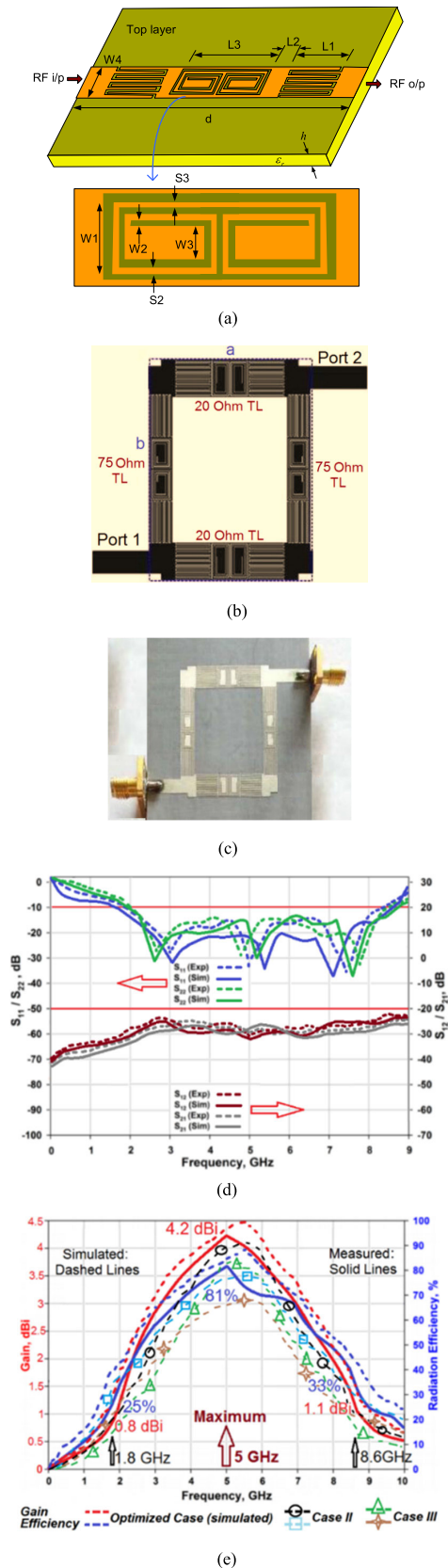
FIGURE 15. (a) CRLH MTM-TL implemented on 50 ohm microstrip line, (b) layout of the CRLH MTM-TL TWA, (c) manufactured prototype, (d) transmission and reflection coefficient responses of the TWA, and (e) TWA's gain and radiation efficiency responses [45].
