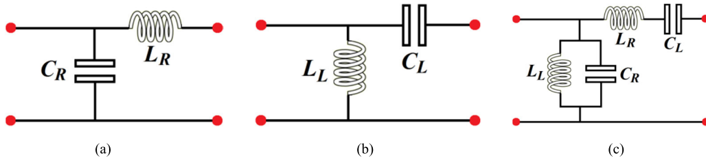
FIGURE 1. Circuit model of the (a) RH transmission line, (b) LH transmission line, and (c) CRLH transmission line.
