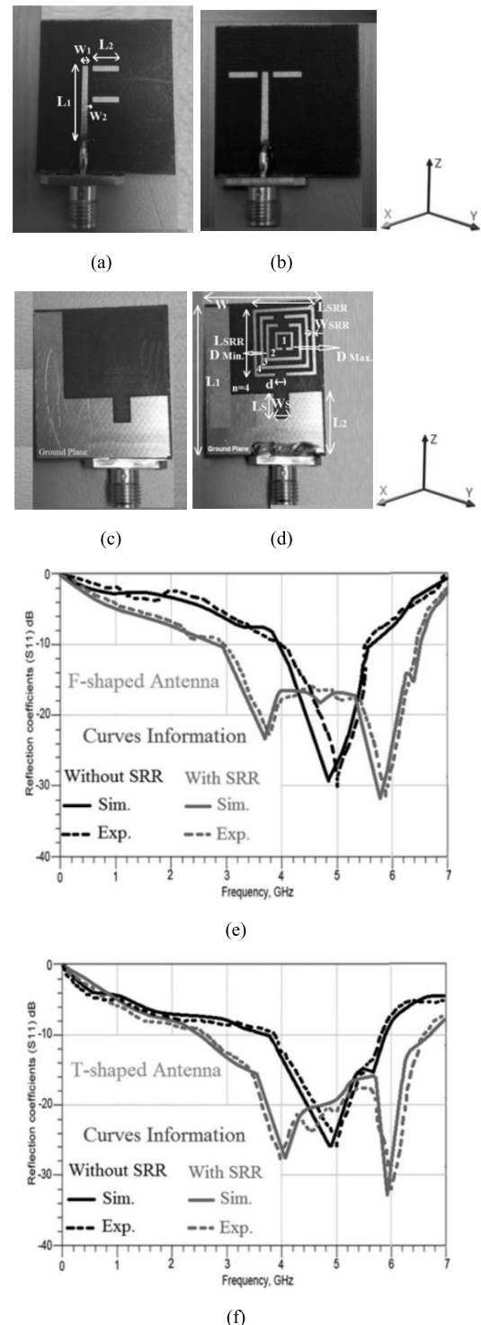
FIGURE 7. Antennas loaded split ring resonators. (a) F-antenna (top-surface), (b) T- antenna (top-surface), (c) bottom-side of both antennas with no split ring resonators, (d) bottom-side of both antennas loaded with split ring resonators, (e) S_{11} \leq -10\text{dB} for the F-antenna, (f) S_{11} \leq -10\text{dB} for the T-antenna, (g) radiation properties for the F-antenna, and (h) radiation properties for the T-antenna [51].
