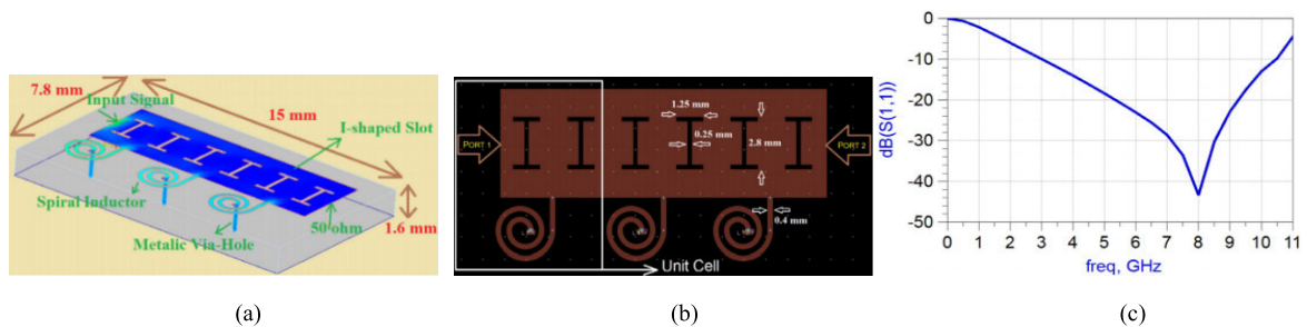
FIGURE 23. UWB MTM antenna with its return loss parameter [39].
