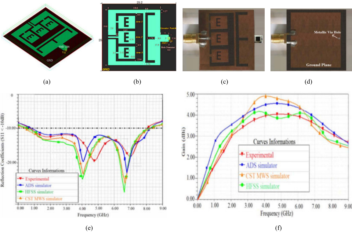
FIGURE 29. Test antenna prototype, its reflection coefficient and gain responses [81].
