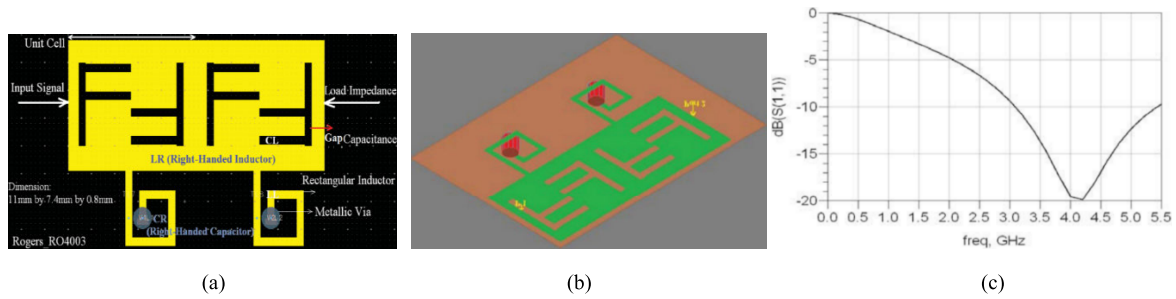
FIGURE 27. CRLH UWB antenna and its reflection coefficient response [43].
