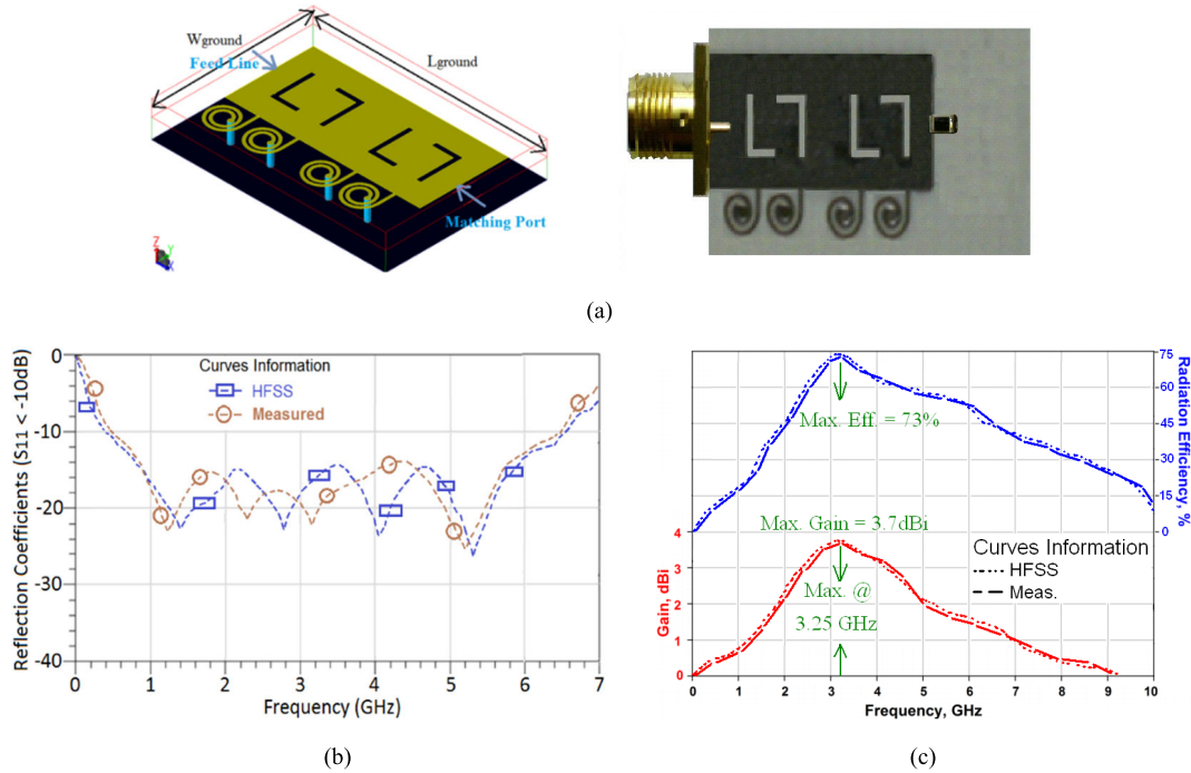
FIGURE 19. (a) Proposed metamaterial based antenna, (b) reflection-coefficient responses, and (c) gain and radiation efficiency curves [35].
