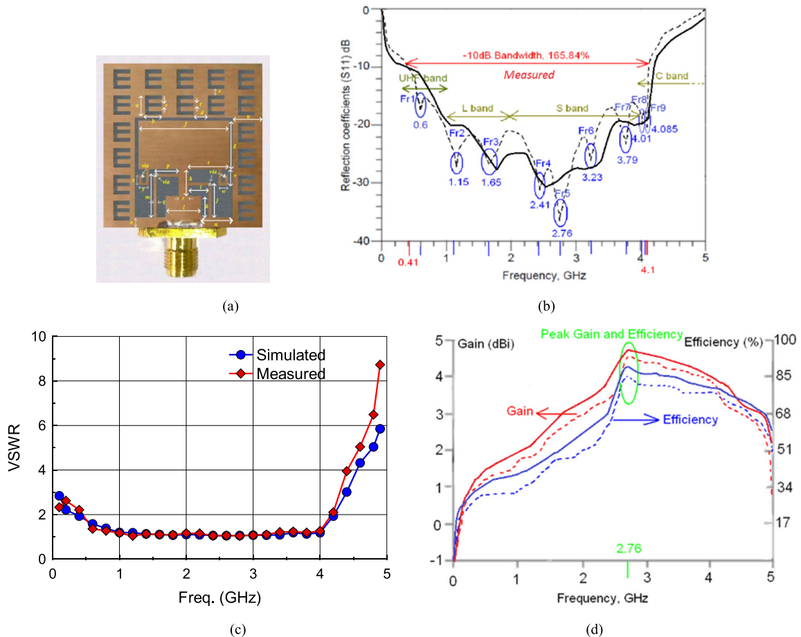
FIGURE 21. (a) Antenna, (b) reflection-coefficient responses, (c) voltage standing wave ratio response, and (d) gain and efficiency responses [37]. Simulated and measured results are presented by solid and dashed lines, respectively.
