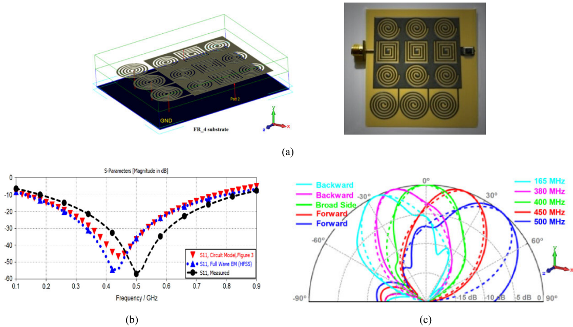
FIGURE 12. (a) Backfire-to-endfire LWA, (b) reflection coefficient responses, and (c) radiation patterns. HFSS: solid lines and experimental: dashed lines [76].
