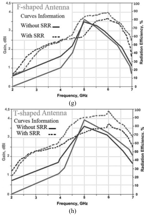
FIGURE 7. (Continued.) Antennas loaded split ring resonators. (a) F-antenna (top-surface), (b) T- antenna (top-surface), (c) bottom-side of both antennas with no split ring resonators, (d) bottom-side of both antennas loaded with split ring resonators, (e) S_{11} \leq -10\text{dB} for the F-antenna, (f) S_{11} \leq -10\text{dB} for the T-antenna, (g) radiation properties for the F-antenna, and (h) radiation properties for the T-antenna [51].
