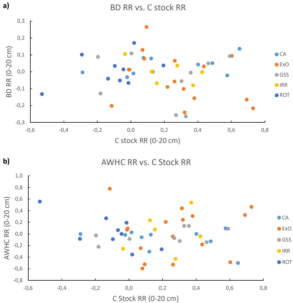
Figure S1. Response ratios of BD (a) and AWHC (b) vs. those observed for soil organic C stock. The five different strategies are represented by colour: conservation agriculture (CA), management of exogenous sources of organic C (ExO), crop rotations (ROT), irrigation (IRR) and optimized grasslands management (GSS).
