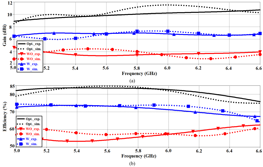
FIGURE 7. Radiation characteristics of the proposed antenna arrays, (a) Gain, and (b) Efficiency. Abbreviation 'WO' and 'W' stand for 'without' and 'with' the EBG and slots, respectively; and 'opt' refers to the optimized array with EBG and slots.
