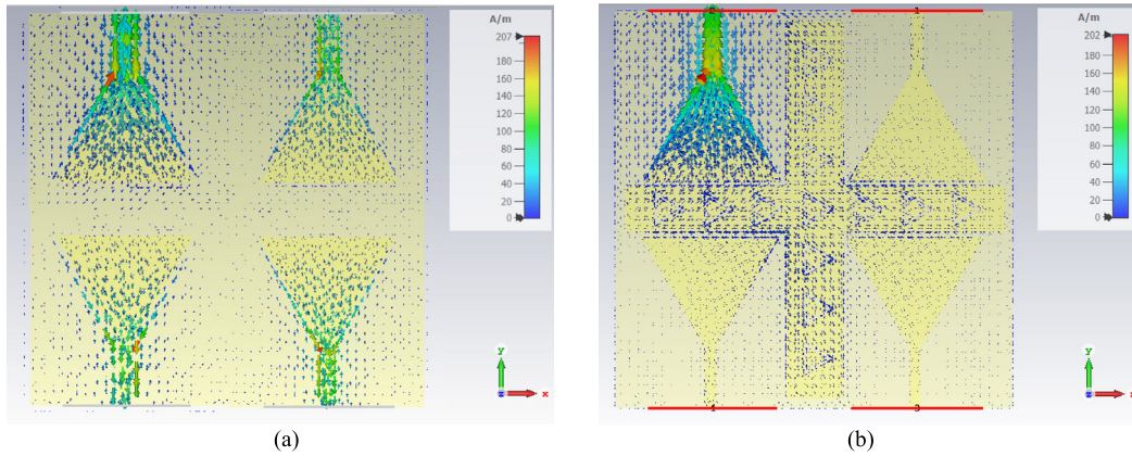
FIGURE 5. (a) Surface current density over the antenna array with no EBG structure when only the top left antenna is excited, and (b) surface current density over the antenna array with the proposed EBG structure.
