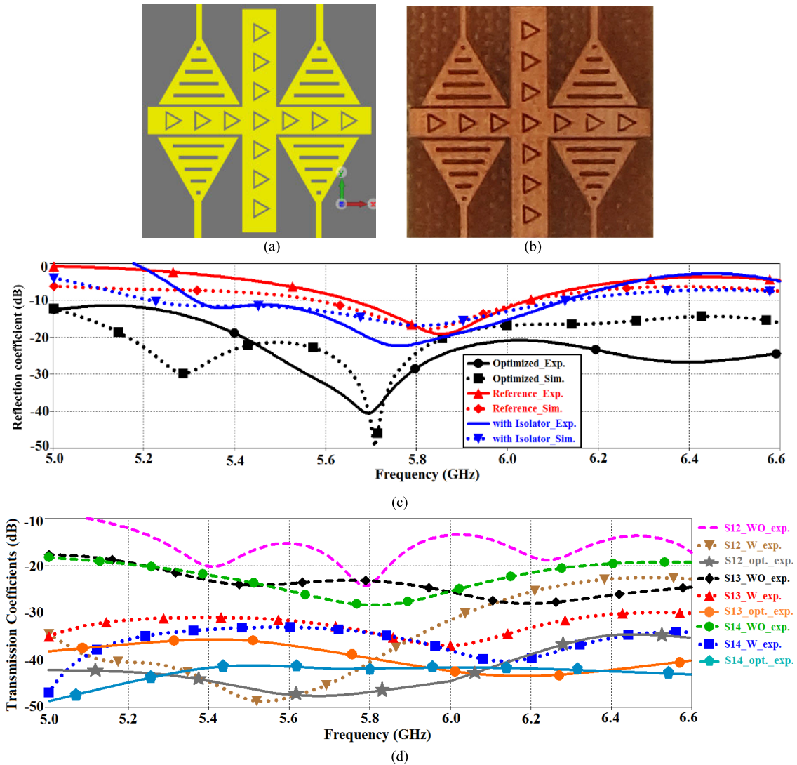
FIGURE 6. The proposed antenna array loaded with metasurface slots, (a) Simulation layout, (b) Photograph of the fabricated array (top side), (c) Array's reflection-coefficient ( S_{11} ) performance, and (d) Isolation response between the radiation patches ( S_{12} , S_{13} & S_{14} ). Abbreviation 'WO' and 'W' stand for 'without' and with 'W' the EBG and slots, respectively; and 'opt' is the optimized array with EBG and slots.
