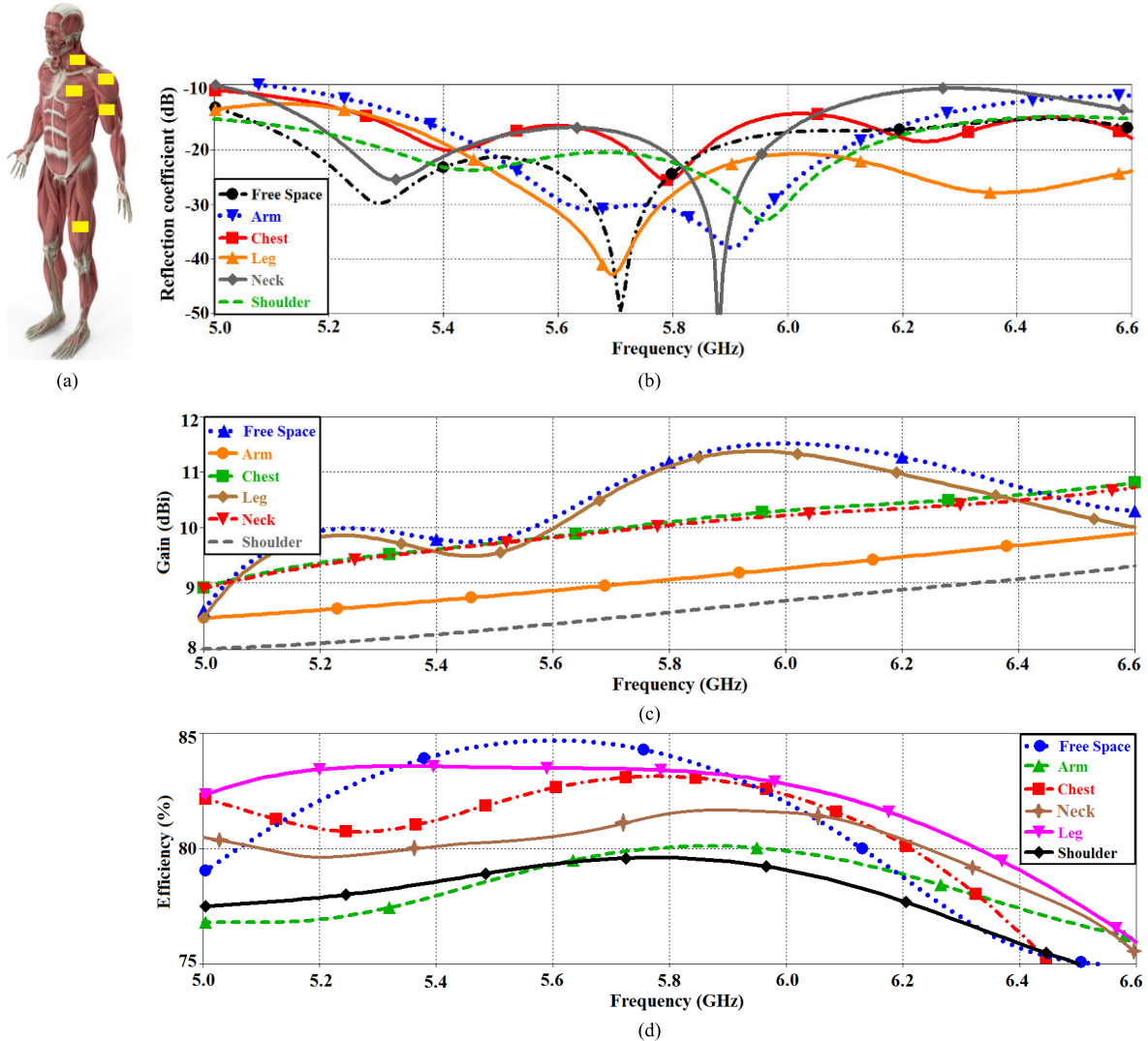
FIGURE 12. Evaluation of the antenna array’s performance when mounted on the human body, (a) array placed at different locations on the human model, (b) on-body loading effect on the array’s reflection-coefficient, (c) on-body loading effects on the array’s radiation gain, and (d) on-body loading effect on the array’s radiation efficiency.
