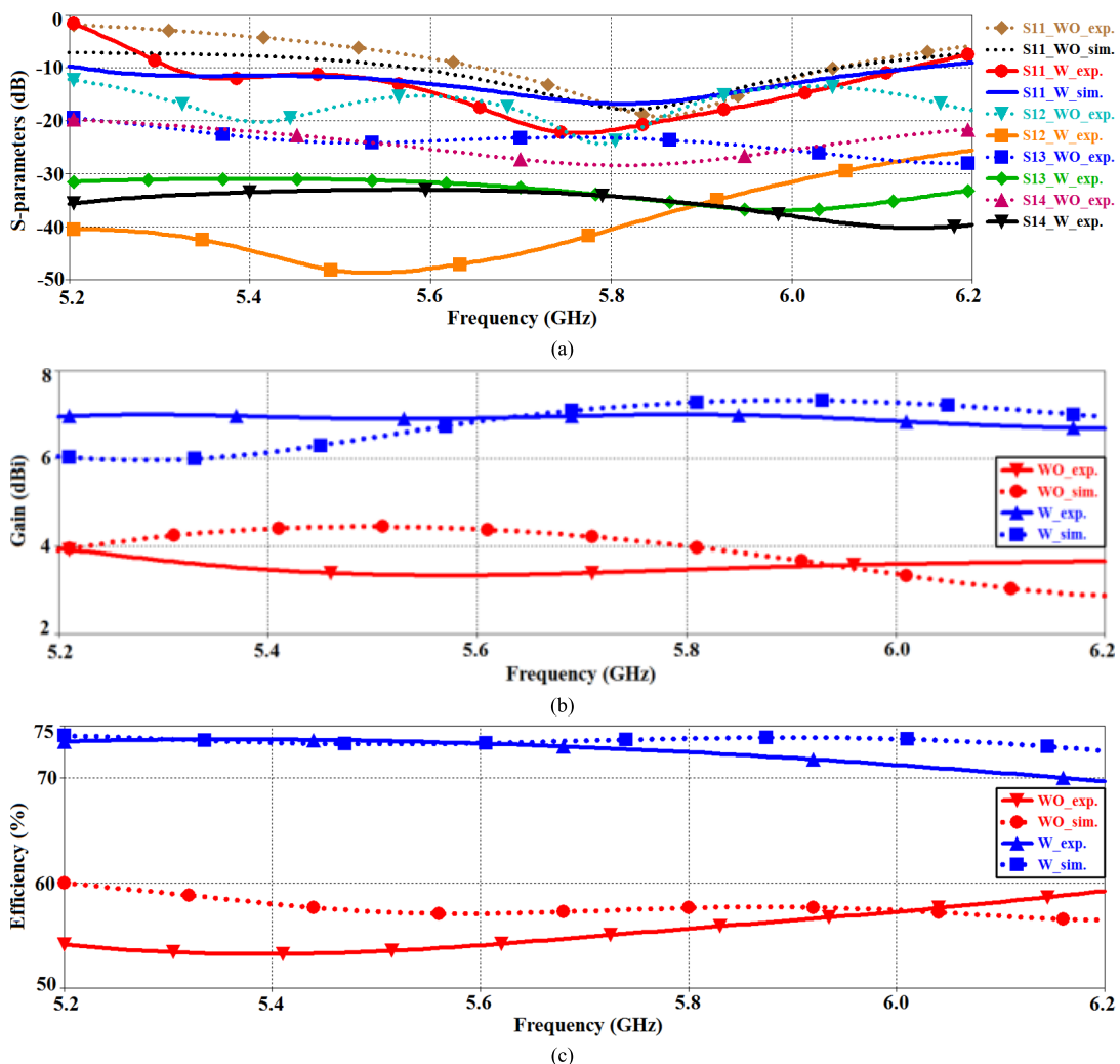
FIGURE 4. Antenna array’s (a) reflection-coefficient ( S_{11} ) & isolation between the patches ( S_{12} , S_{13} & S_{14} ), (b) Gain as a function of frequency, & (c) Radiation efficiency as a function of frequency. Note, the abbreviations ‘WO’ stands for ‘without’ the EBG decoupling structure, and ‘W’ stands for ‘with’ the decoupling structure.
