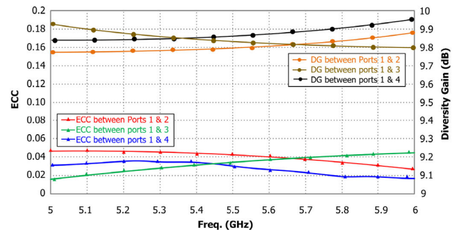
FIGURE 13. The measured envelop correlation coefficient (ECC) and diversity gain (DG) of the proposed 2 \times 2 element antenna array.
