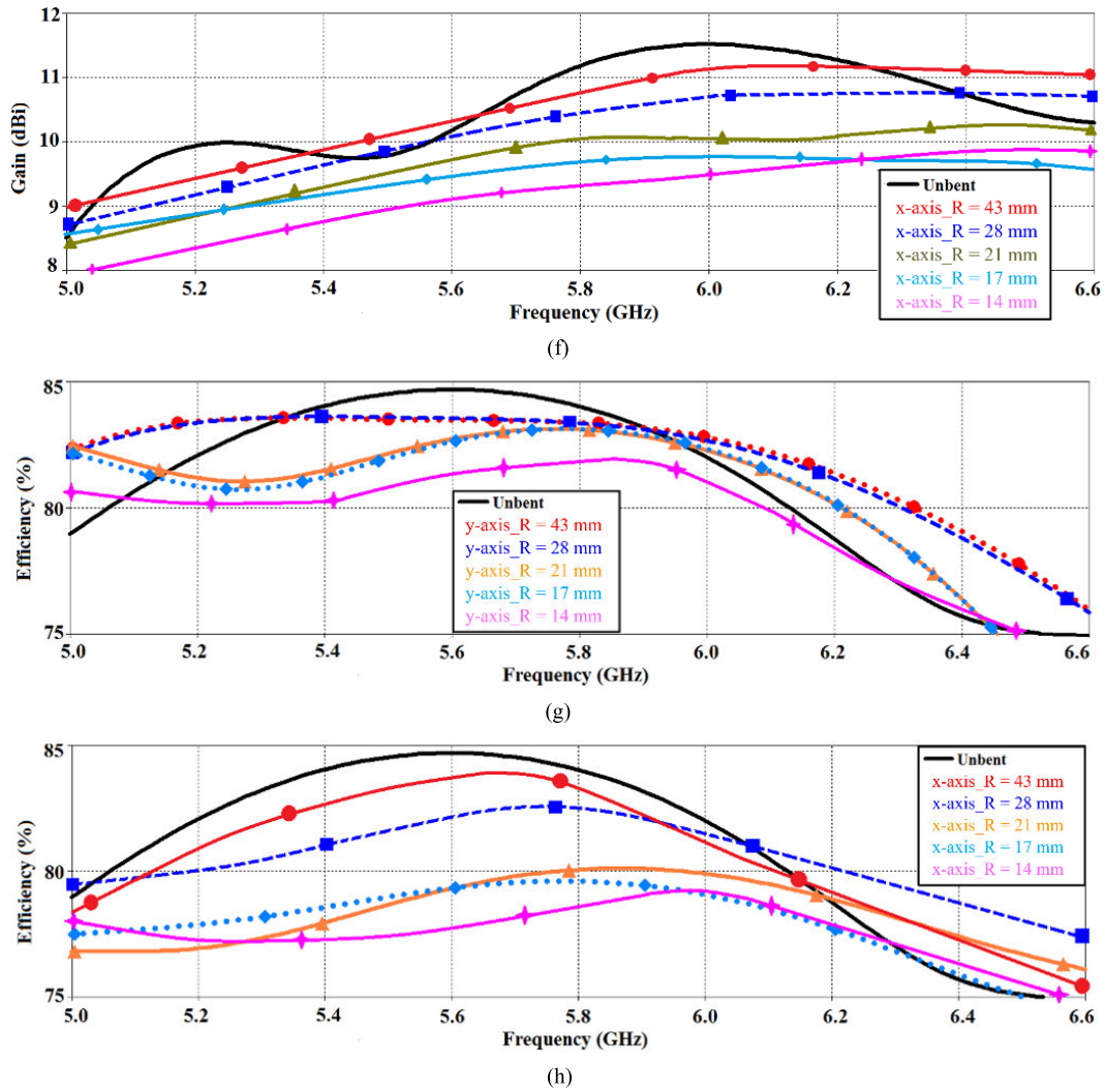
FIGURE 11. (Continued.) Deformation of the antenna array and its performance, (a) bending in the yz-plane, (b) bending in the xz-direction, (c) reflection-coefficients for various bend radii in the yz-plane, (d) reflection-coefficients for various bend radii in the xz-plane, (e) gain at various bend radii in the yz-plane, (f) gain at various bend radii in xz-plane, (g) radiation efficiency at various bend radii in the yz-plane, and (h) radiation efficiency at various bend radii in xz-plane.
