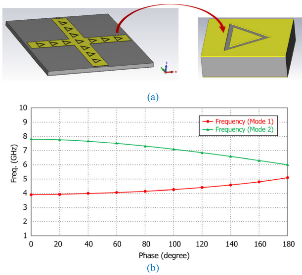
FIGURE 3. (a) The proposed EBG decoupling structure, and (b) dispersion diagram of the EBG structure obtained by CST microwave studio.
