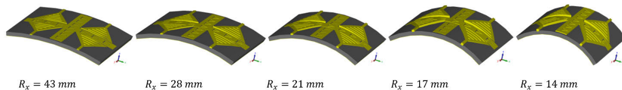
(b) xz-plane bending radius
