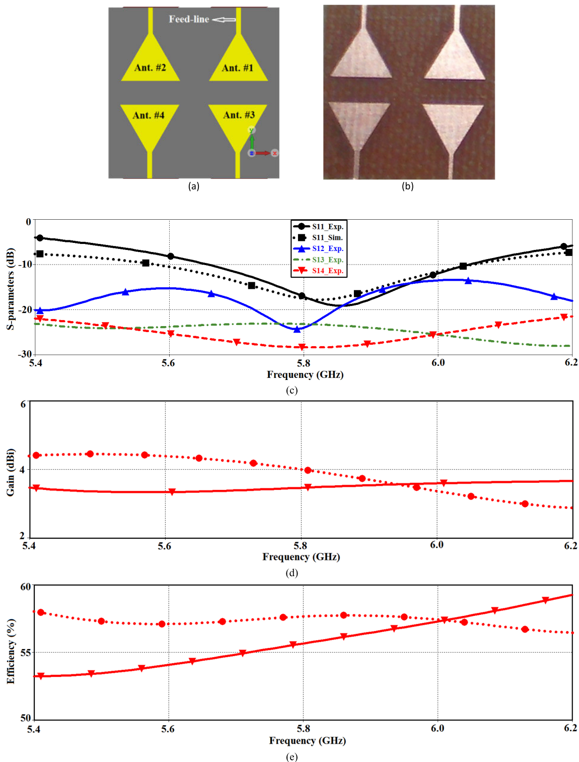
FIGURE 1. Reference 2 \times 2 antenna array, (a) simulation layout, (b) photograph of the fabricated array (top side), (c) array's reflection-coefficient ( S_{11} ) & isolation between the patches ( S_{12} , S_{13} & S_{14} ), (d) antenna gain as a function of frequency, & (e) radiation efficiency as a function of frequency.
