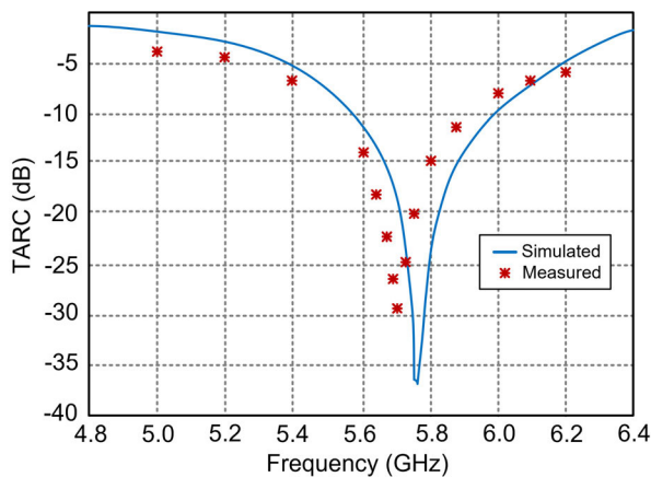
FIGURE 14. The simulated and measured TARC of the proposed 2 × 2 element antenna array.
