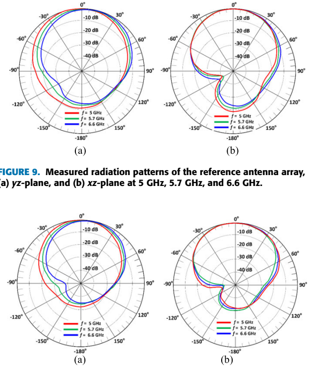
FIGURE 10. Measured radiation patterns the proposed antenna array with EBG decoupling structure and metasurface slots in (a) yz-plane, and (b) xz-plane at 5 GHz, 5.7 GHz, and 6.6 GHz.
