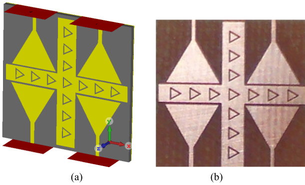
FIGURE 2. (a) simulation layout of the 2 \times 2 antenna array loaded with EBG decoupling structure, (b) photograph of the fabricated array (top side).
