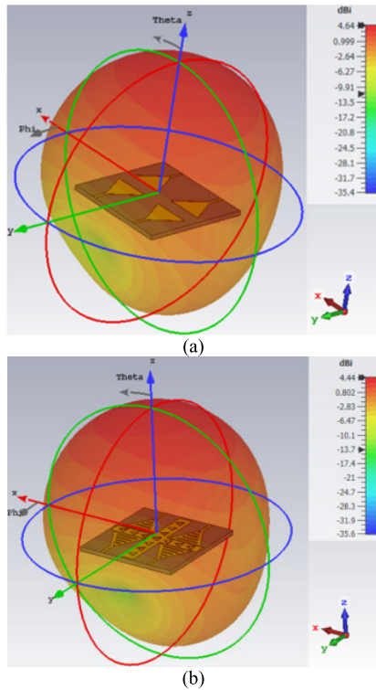
FIGURE 8. Simulated far-field radiation of the proposed antenna array (a) reference array, and (b) array with EBG decoupling structure and metasurface slots.
