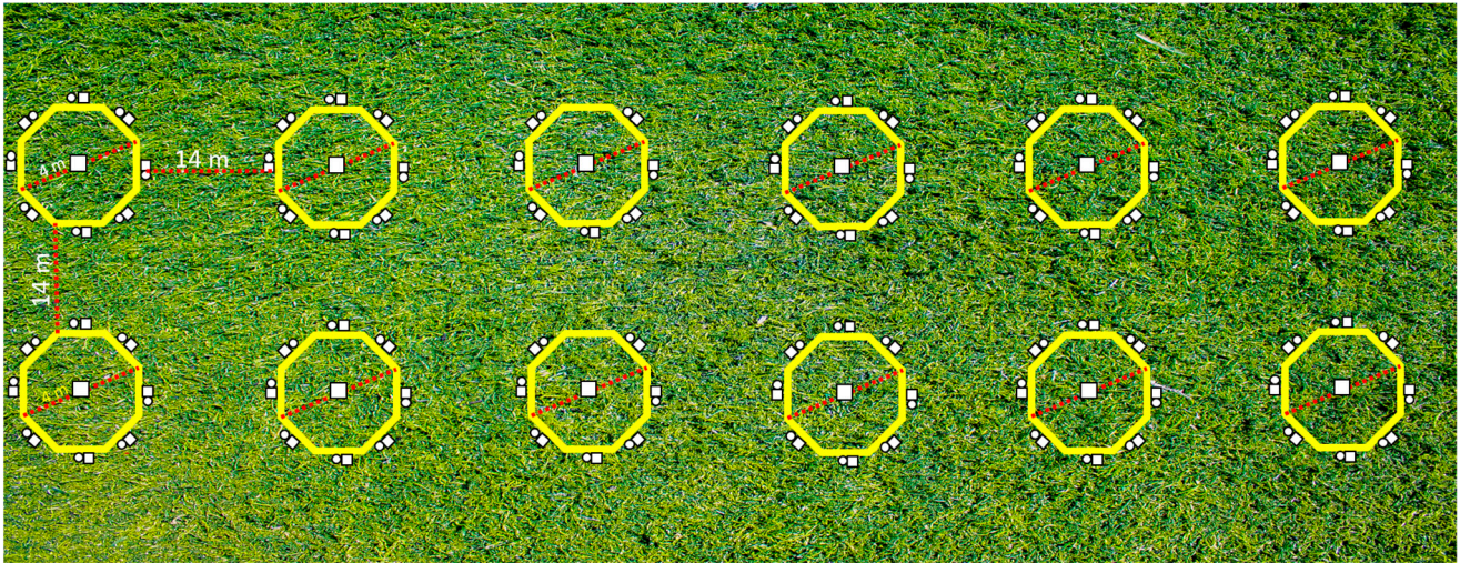
Figure S1. Design of mini-FACE experimental showing distribution of rings into field. Source: Own elaboration.
