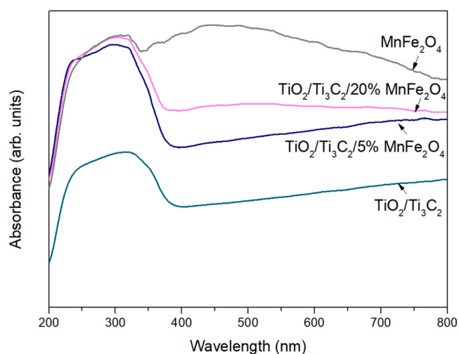
Fig. 4. The DR/UV-vis spectra for prepared materials.
