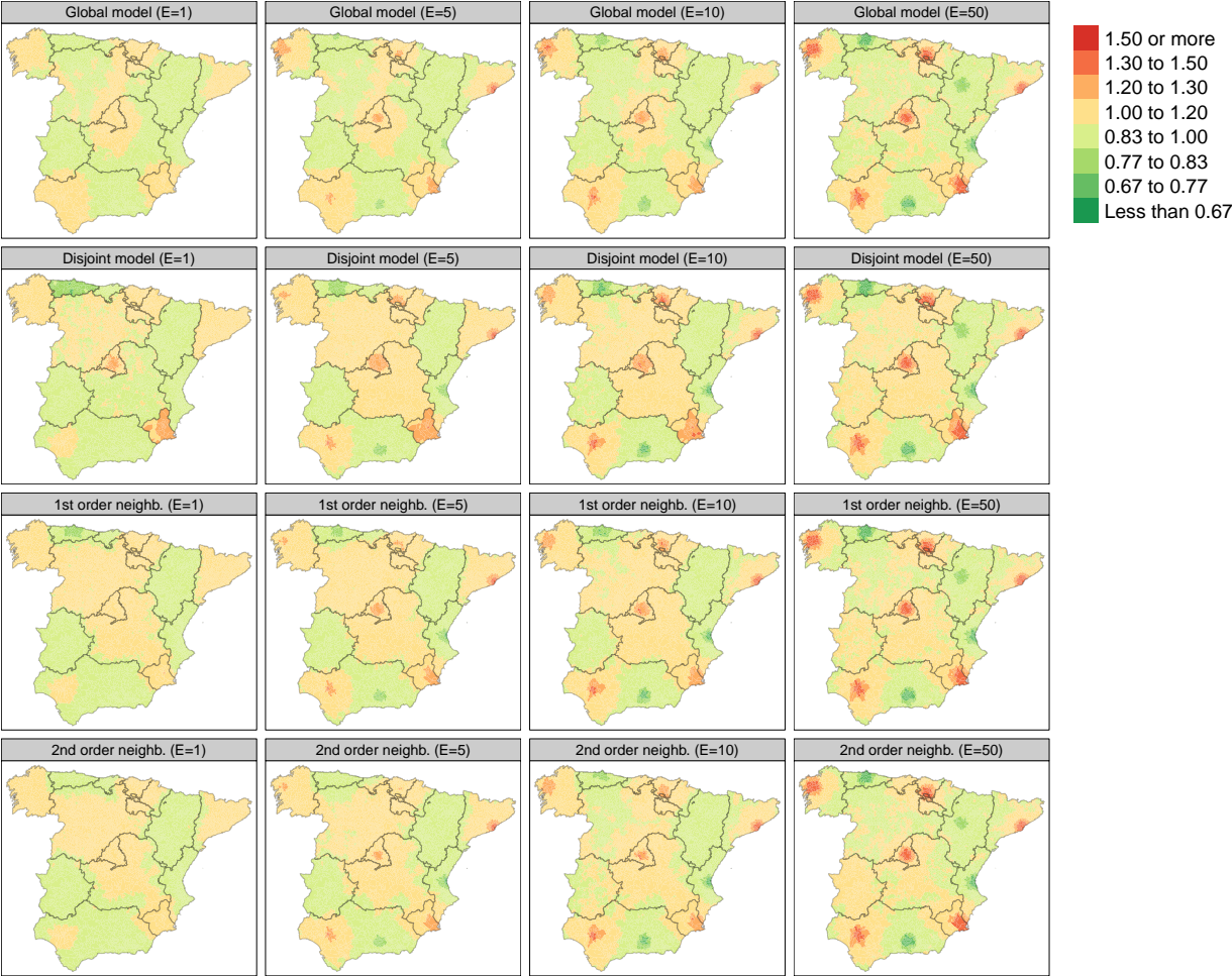
Figure 1: Average values of the relative risks r_i posterior median estimates for the simulation study of Scenario 1.
