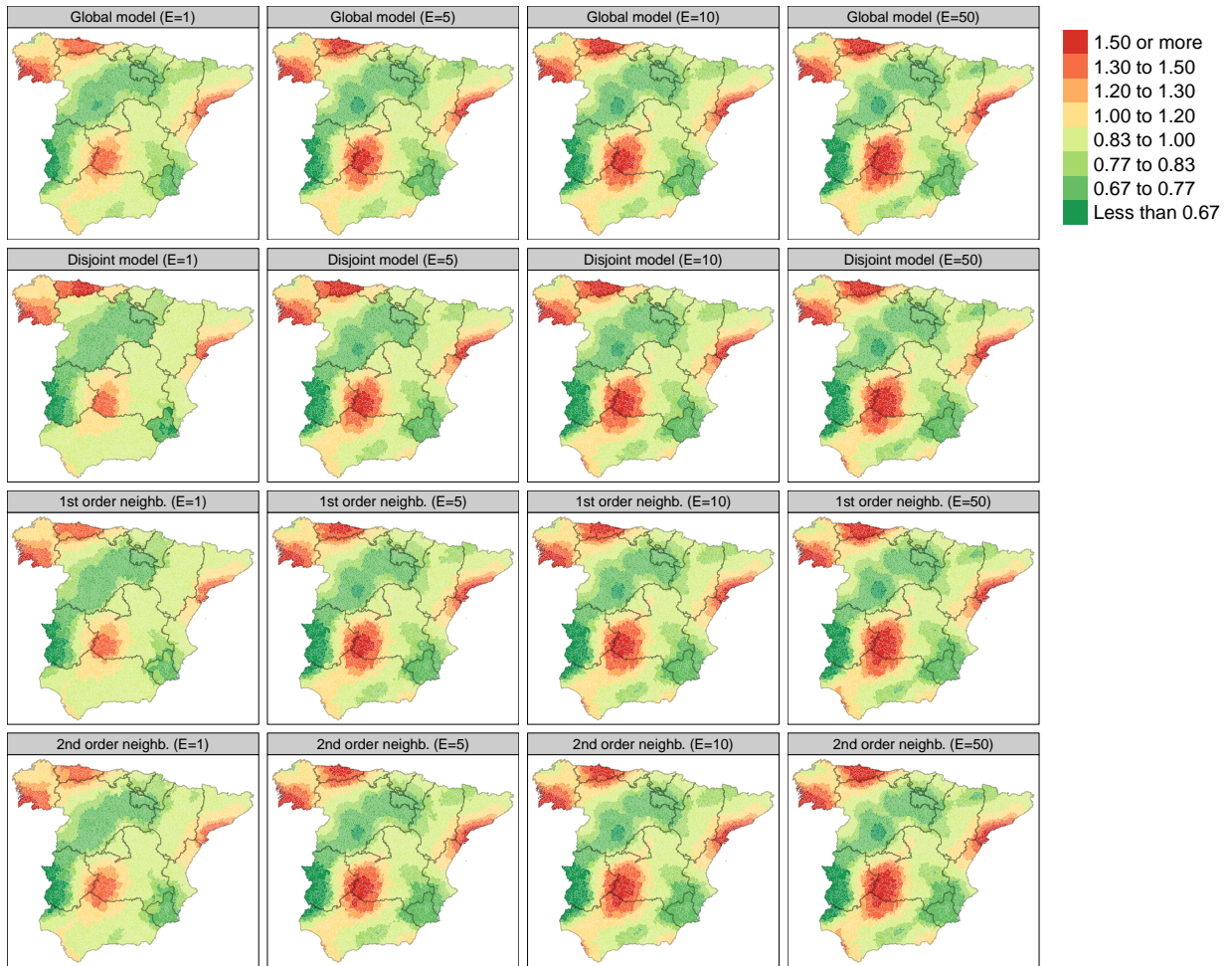
Figure 2: Average values of the relative risks r_i posterior median estimates for the simulation study of Scenario 2.
